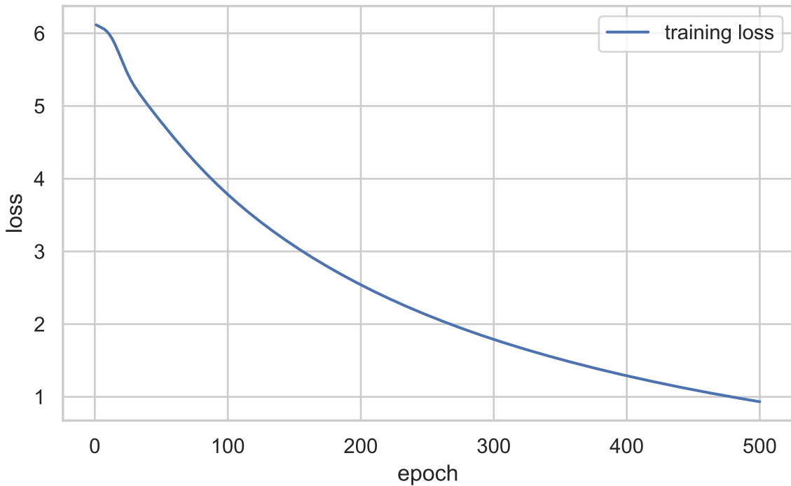
CBOW 10-D training loss
