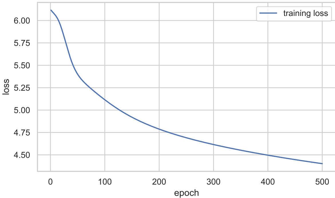
CBOW 2-D training loss
