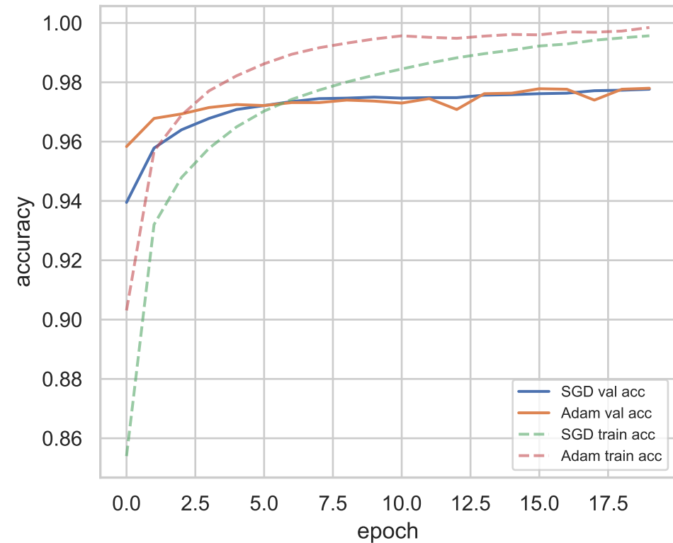
MNIST accuracy
