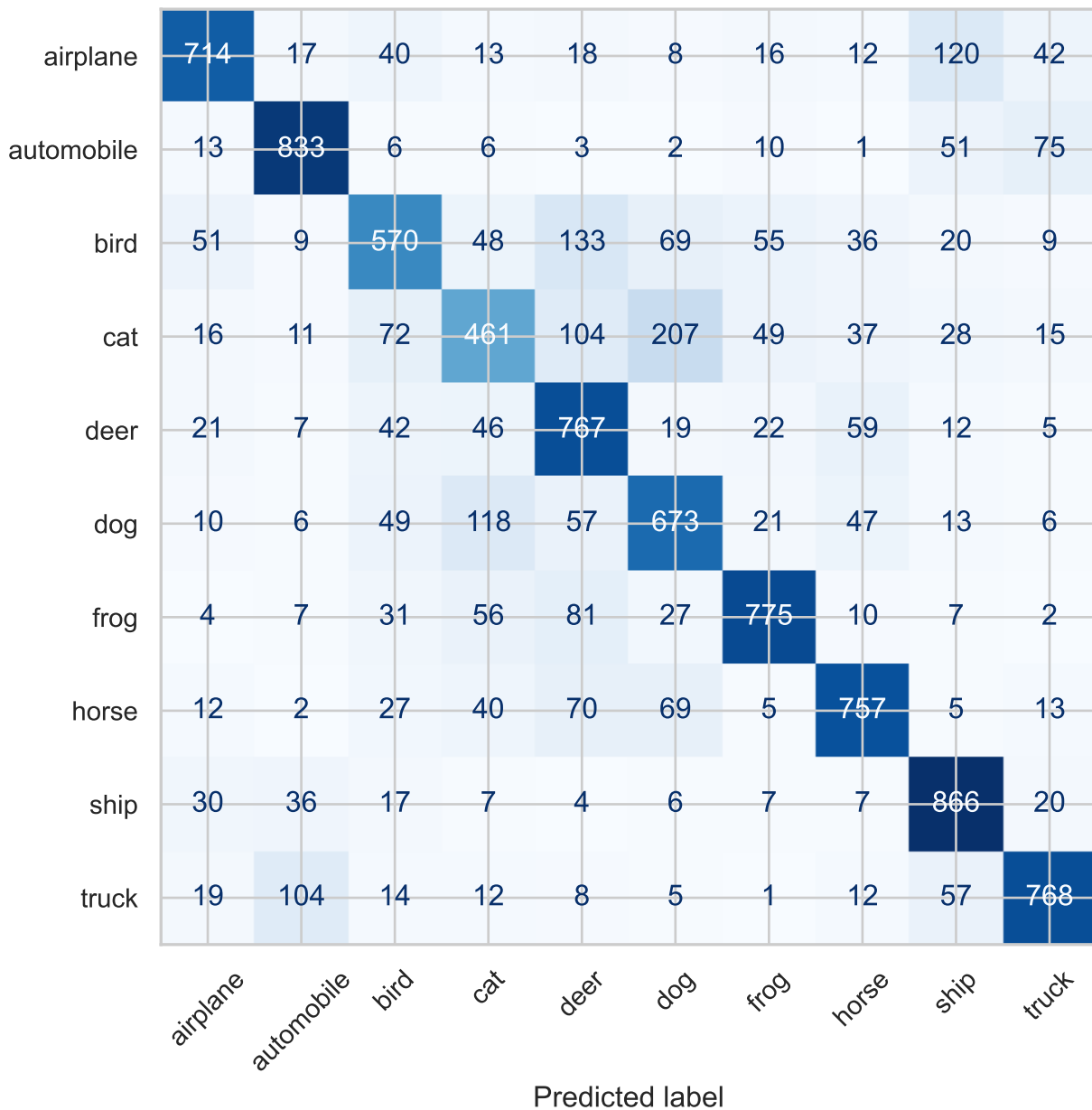
CIFAR-10 confusion matrix
