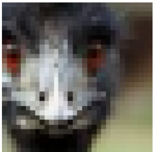
T:bird\nP:ship
