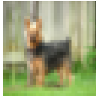
T:dog\nP:deer
