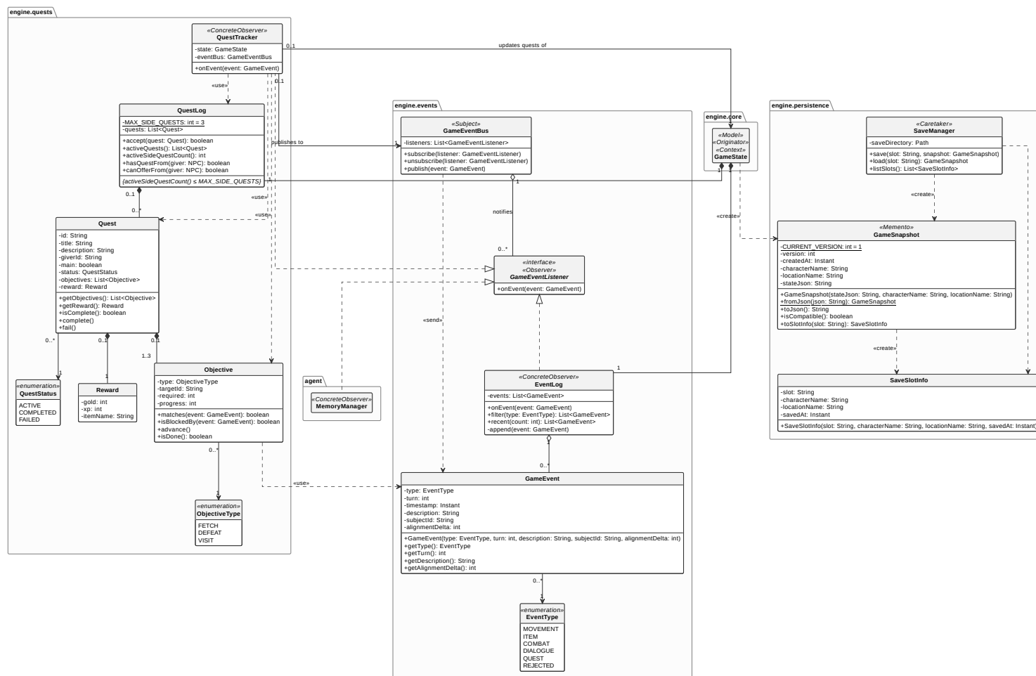
Class Diagram 5 — Quests, Events and Persistence (Observer, Memento)
