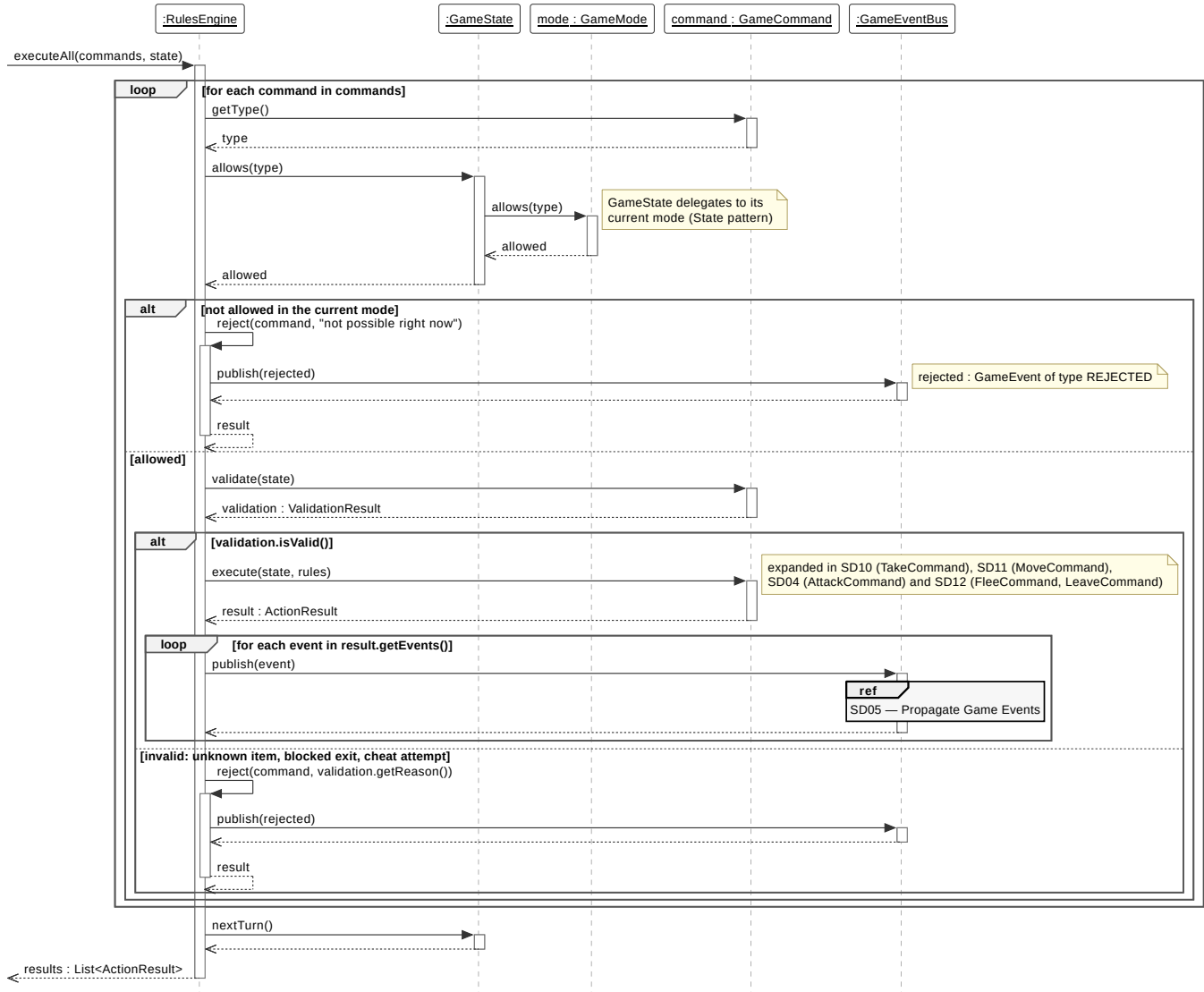
SD03 — Execute Game Commands (Command, State) referenced by SD02, SD04, SD07 and SD10-SD12
