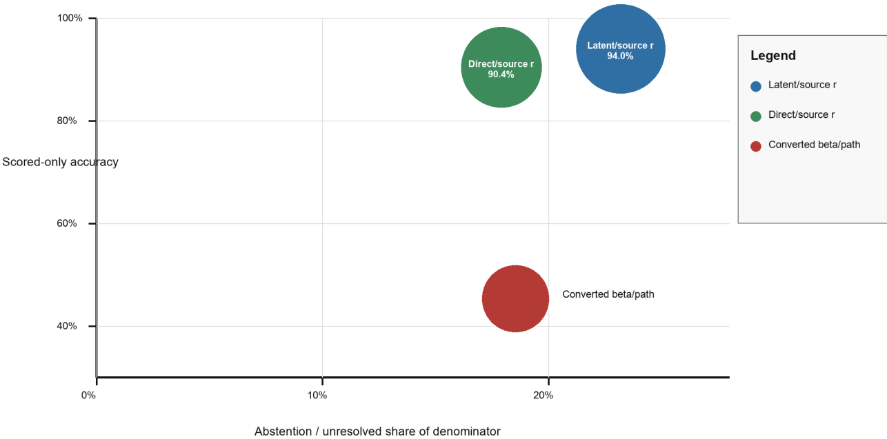
Figure 3 | Accuracy and review-burden profile
