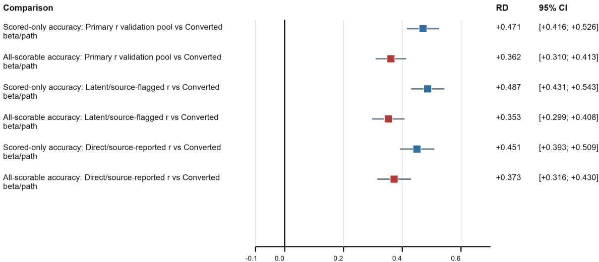
Figure 2 | Accuracy difference against the converted beta/path sensitivity stratum
