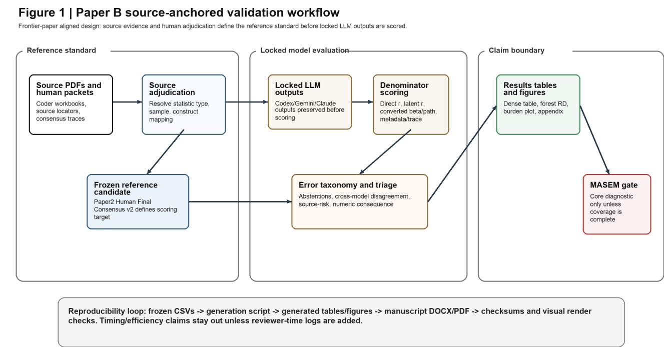
Figure 1. Source-anchored validation workflow
