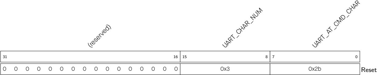
Register 26.31. UART_AT_CMD_CHAR_REG (0x005C)
