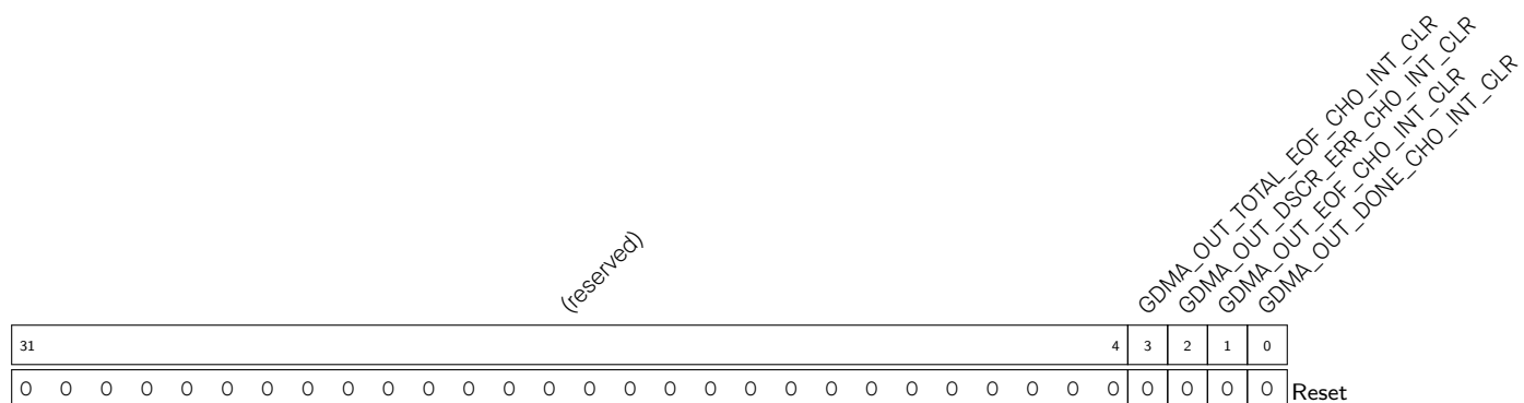
Register 3.18. GDMA_OUT_INT_CLR_CH n _REG ( n : 0-4) (0x0074+192* n )
