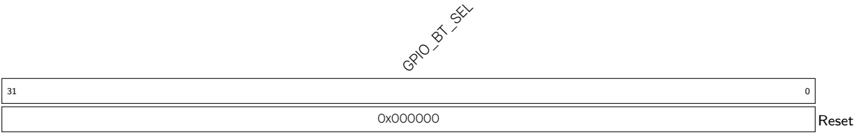
Register 6.1. GPIO_BT_SELECT_REG (0x0000)
