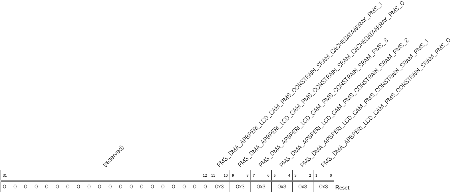
Register 15.25. PMS_DMA_APBPERI_LCD_CAM_PMS_CONSTRIN_1_REG (0x0094)
