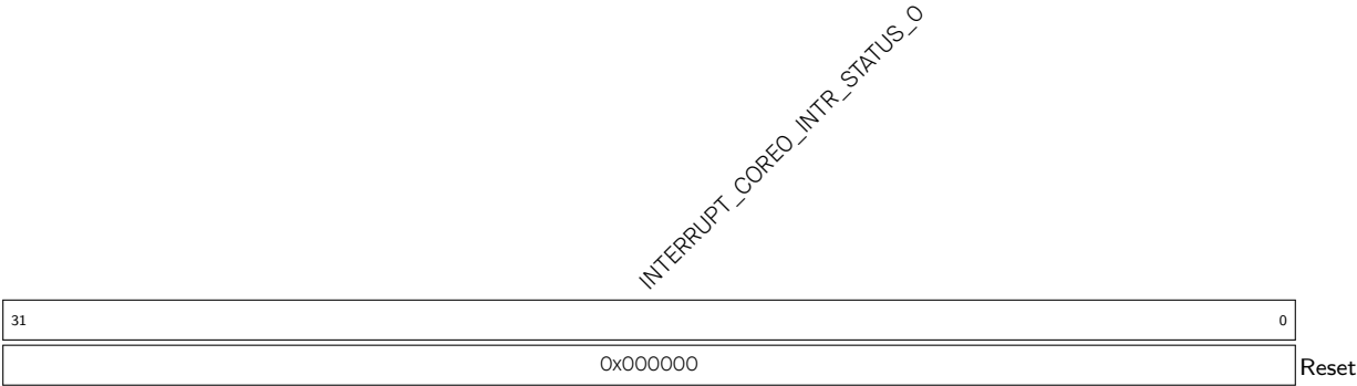
Register 9.85. INTERRUPT_CORE0_INTR_STATUS_0_REG (0x018C)
