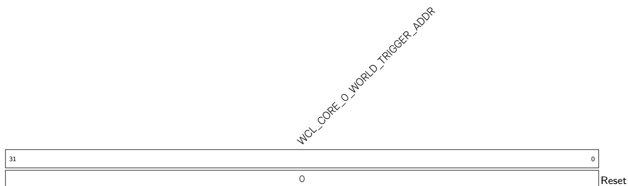
Register 16.8. WCL_CORE_0_World_TRIGGER_ADDR_REG (0x0140)
