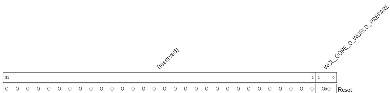
Register 16.9. WCL_CORE_0_World_PREPARE_REG (0x0144)
