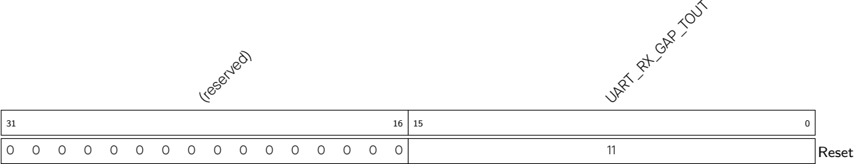
Register 26.30. UART_AT_CMD_GAPTOUT_REG (0x0058)
