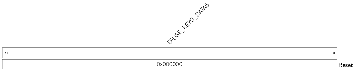
Register 5.45. EFUSE_RD_KEYO_DATA5_REG (0x00B0)
