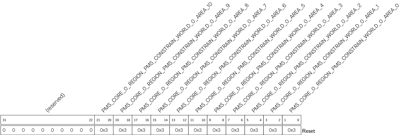
Register 15.58. PMS_CORE_0_REGION_PMS_CONSTRAIN_1_REG (0x0164)
