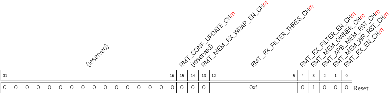
Register 37.5. RMT_CHmCONF1_REG (m = 4, 5, 6, 7) (0x0034, 0x003C, 0x0044, 0x004C)
