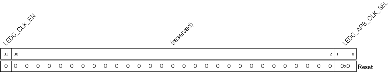
Register 35.3. LEDC_CONF_REG (0x00D0)
