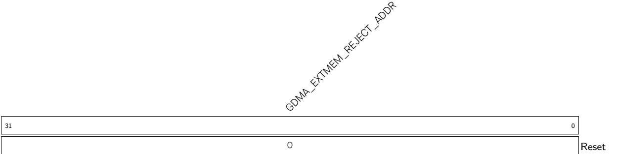
Register 3.41. GDMA_EXTMEM_REJECT_ADDR_REG (0x03F4)
