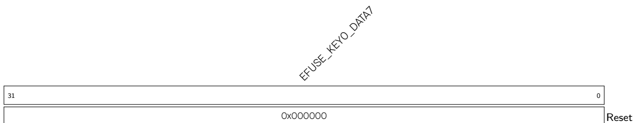
Register 5.47. EFUSE_RD_KEYO_DATA7_REG (0x00B8)
