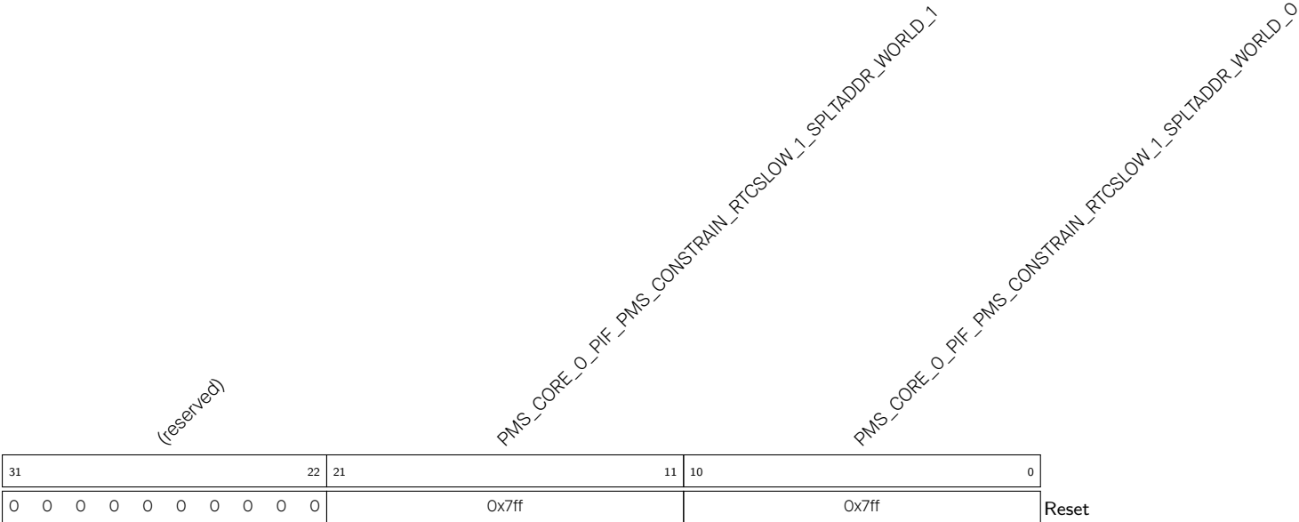
Register 15.55. PMS_CORE_0_PIF_PMS_CONSTRRAIN_13_REG (0x0158)
