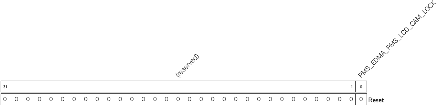
Register 15.82. PMS_EDMA_PMS_LCD_CAM_LOCK_REG (0x02E0)
