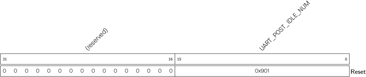
Register 26.29. UART_AT_CMD_POSTCNT_REG (0x0054)
