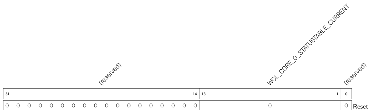
Register 16.7. WCL_CORE_0_STATUSTABLE_CURRENT_REG (0x00FC)
