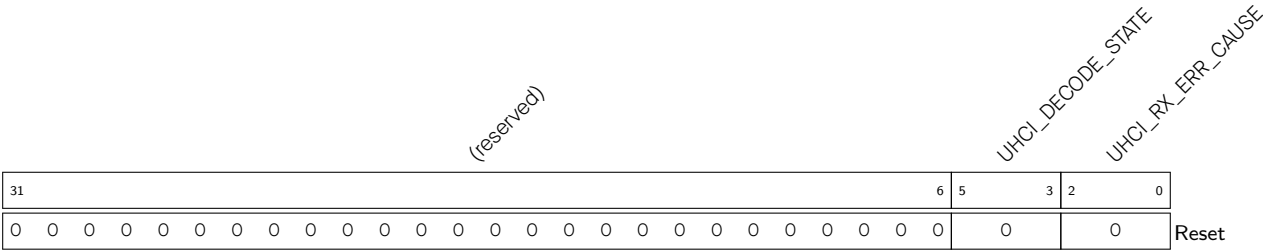
Register 26.64. UHCI_STATE0_REG (0x001C)
