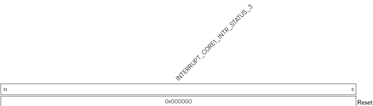
Register 9.178. INTERRUPT_CORE1_INTR_STATUS_3_REG (0x0998)
