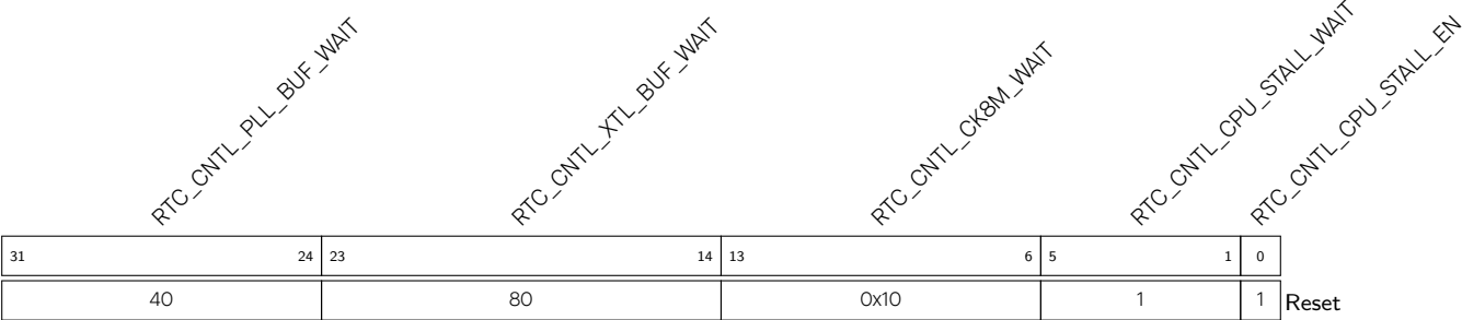
Register 10.8. RTC_CNTL_RTC_TIMER1_REG (0x001C)
