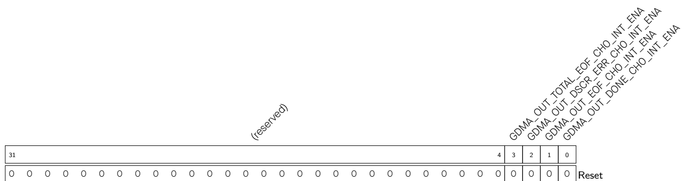
Register 3.17. GDMA_OUT_INT_ENA_CH n _REG ( n : 0-4) (0x0070+192* n )
