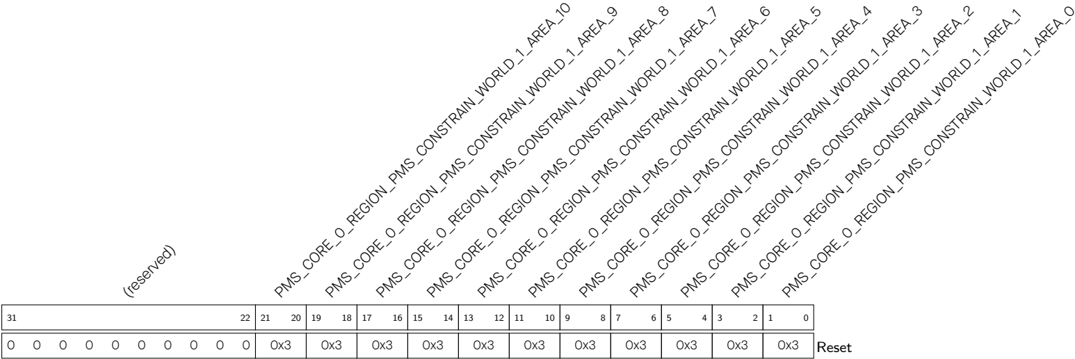
Register 15.59. PMS_CORE_0_REGION_PMS_CONSTRIN_2_REG (0x0168)
