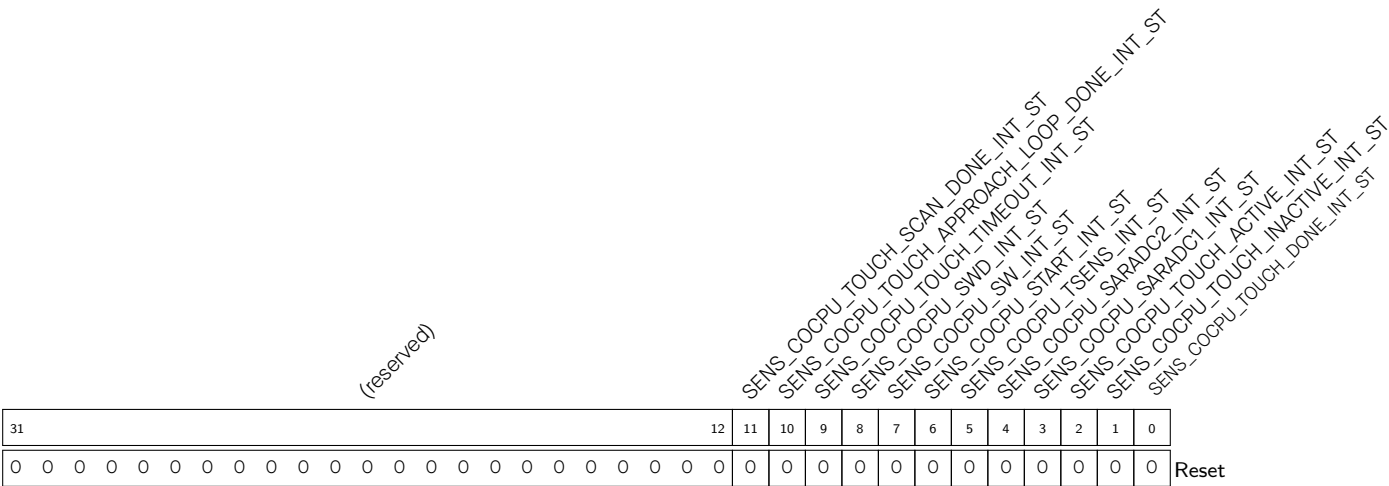
Register 2.7. SENS_SAR_COCPU_INT_ST_REG (0x00F0)
