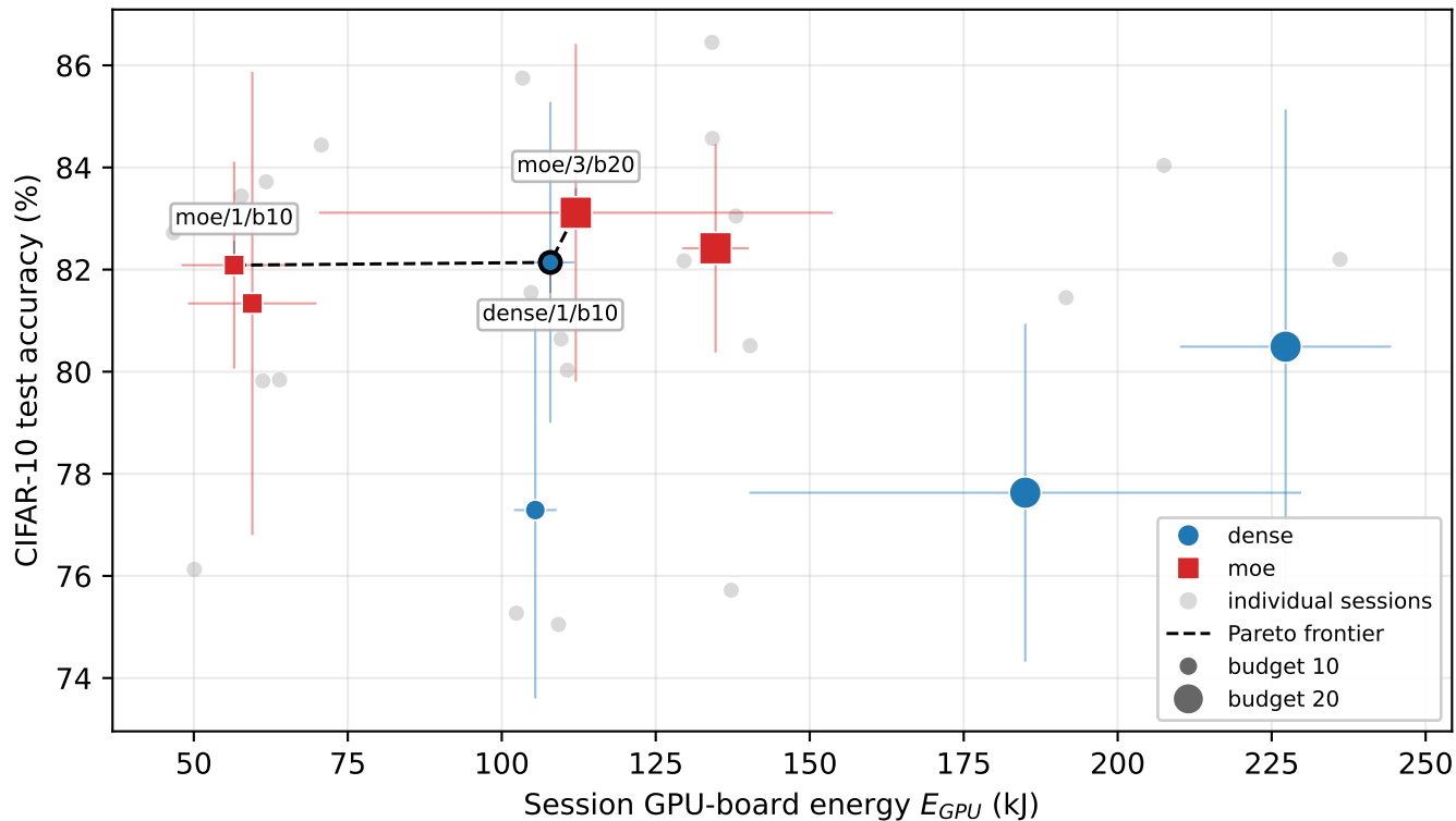
Energy/accuracy Pareto frontier
