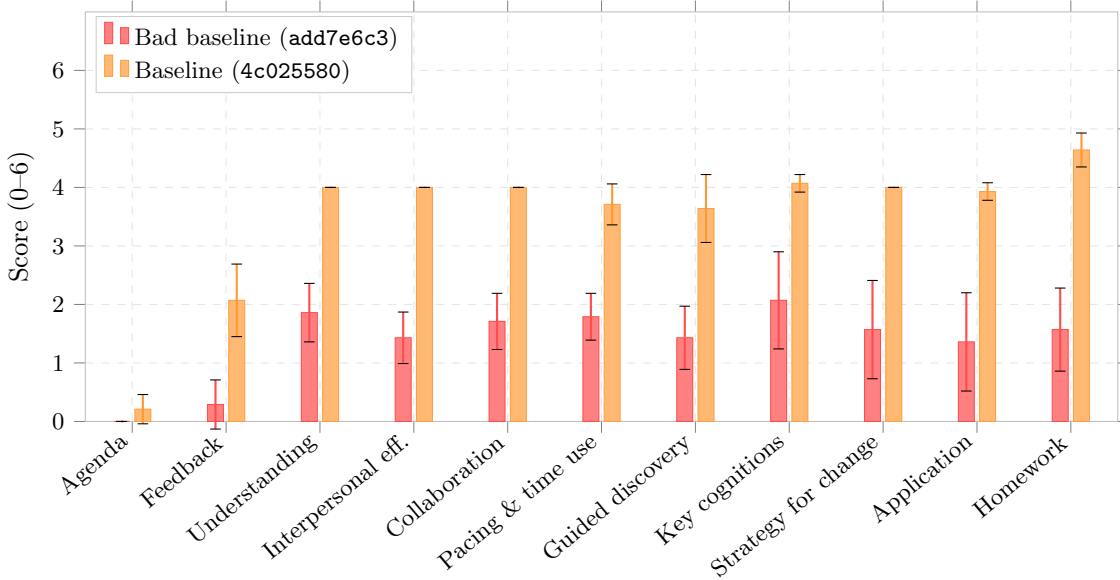
Figure 8.1: CTRS item scores (raw, 0–6 scale) for the bad baseline (add7e6c3) vs. baseline (4c025580), n = 14 persona conversations each. Error bars show 95% CIs via t -distribution ( df = 13 ).
