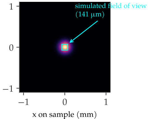
focused spot, d = 4 \mu\text{m}
