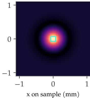
clipped (default), d = 1 \mu\text{m}
