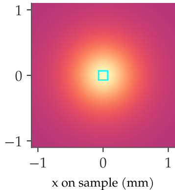
point source, d = 0.4 \mu\text{m}
