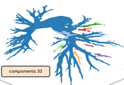
Topology-Only
