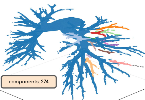
Anatomy-Only
