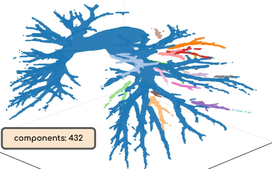
Baseline Segmentation
