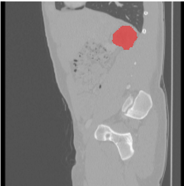
Ground Truth
