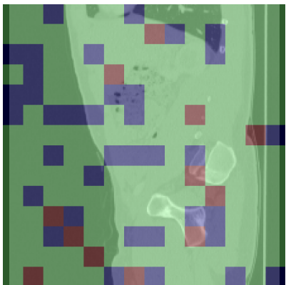
Transformer Head 3
