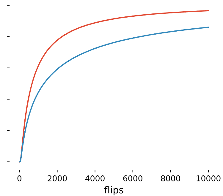
dataset = ruf75-320
