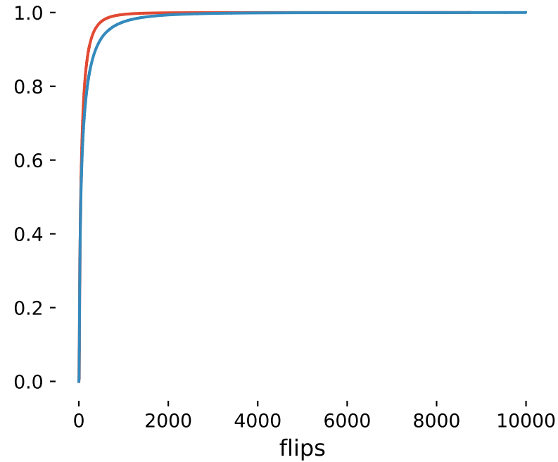
dataset = ruf20-91
