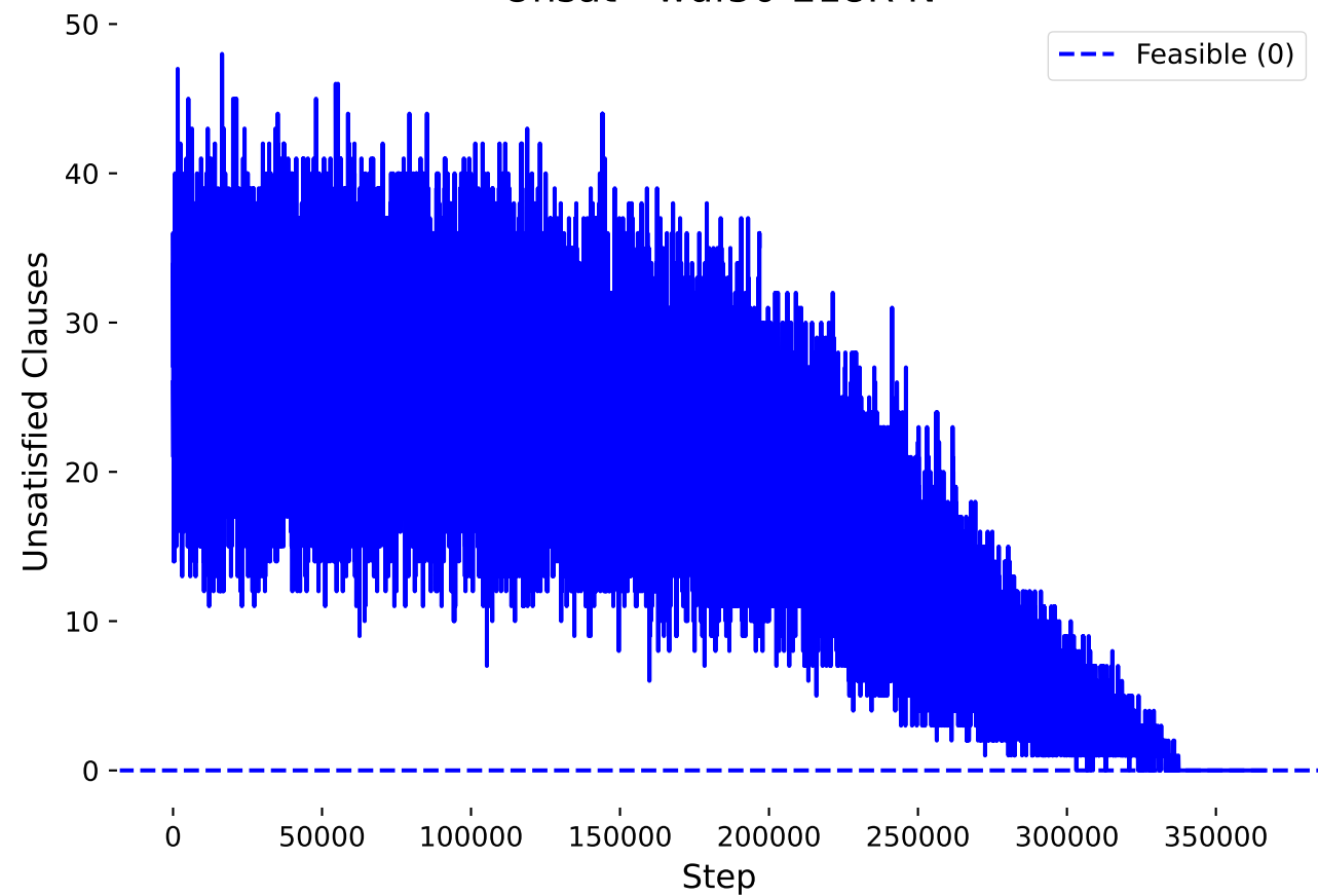
Unsat - wuf50-218R-N
