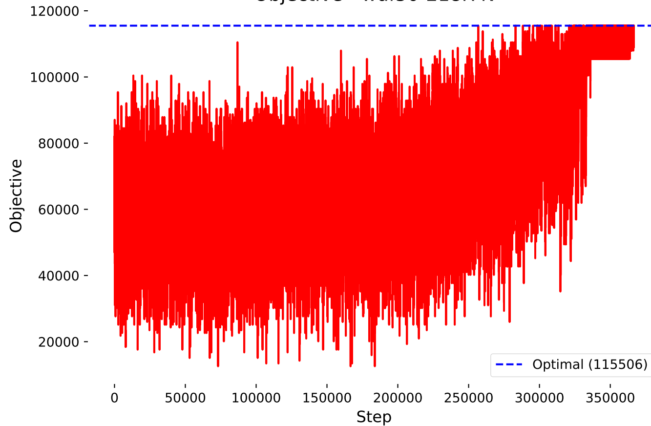
Objective - wuf50-218R-N
