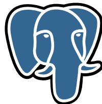
Figure 8: PostgreSQL logo
