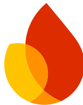
Figure 6: Firebase logo
