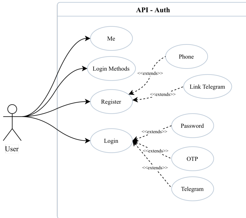
Figure 3: User account use case diagram
