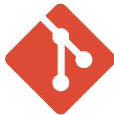
Figure 16: Git logo
