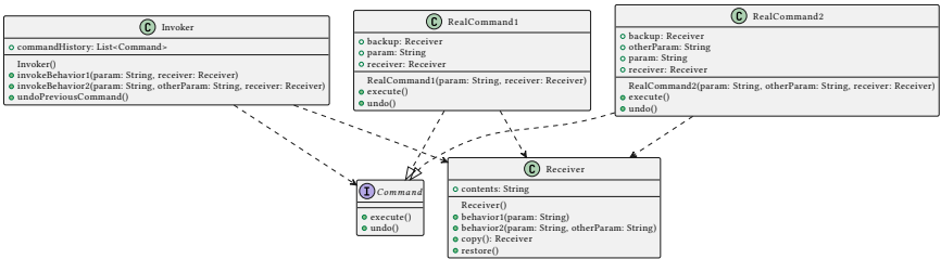
Figure 48: command example
