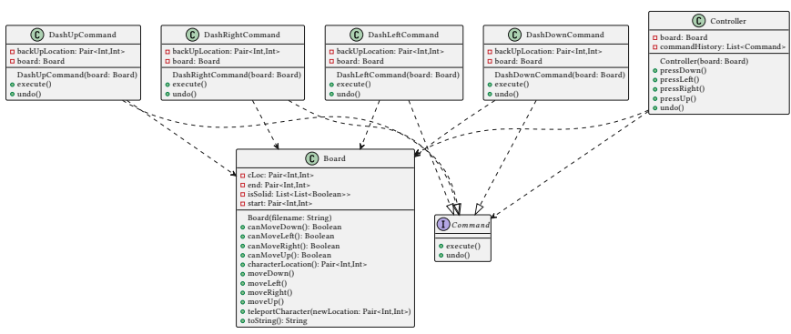
Figure 49: command example
