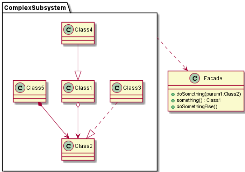
Figure 38: facade
