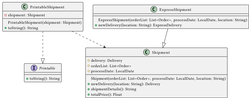
Figure 35: adapter example
