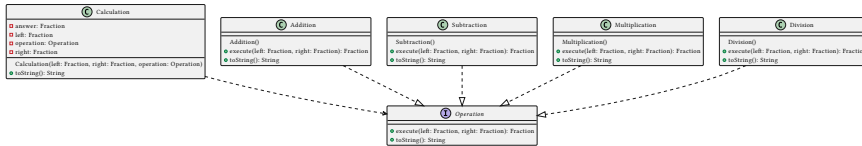
Figure 41: strategy pattern example
