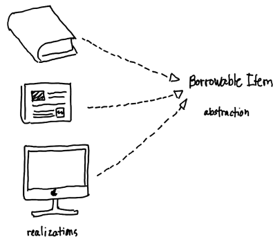
Figure 17: Realization Relationship Example
