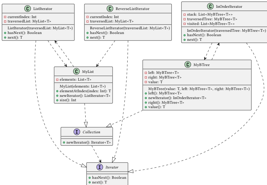
Figure 57: iterator
