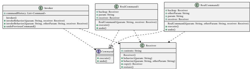
Figure 48: command example
