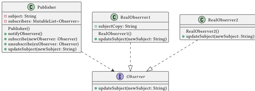
Figure 51: observer
