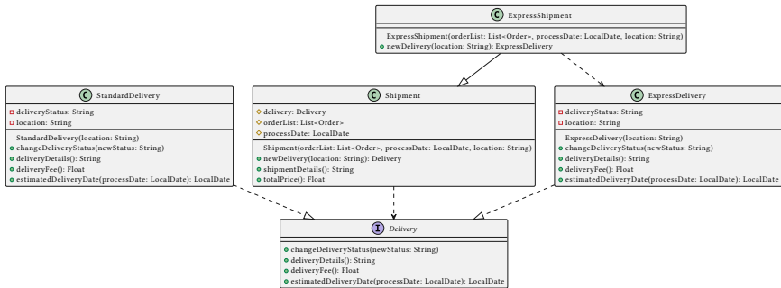
Figure 25: online marketplace
