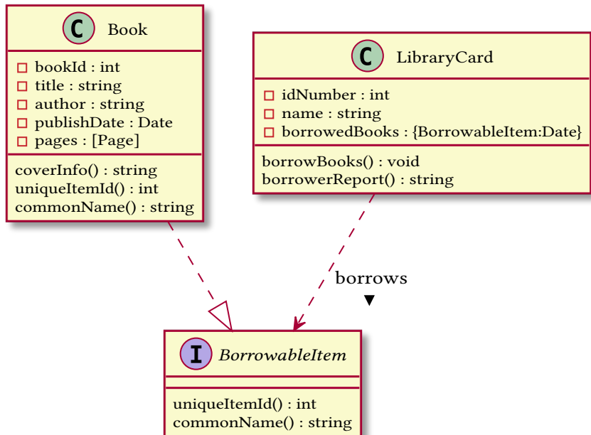
Figure 8: Class diagram of a book class
