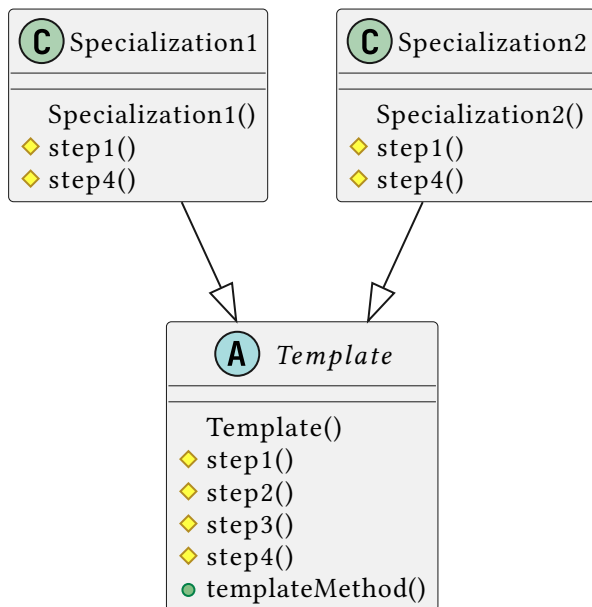
Figure 54: template method
