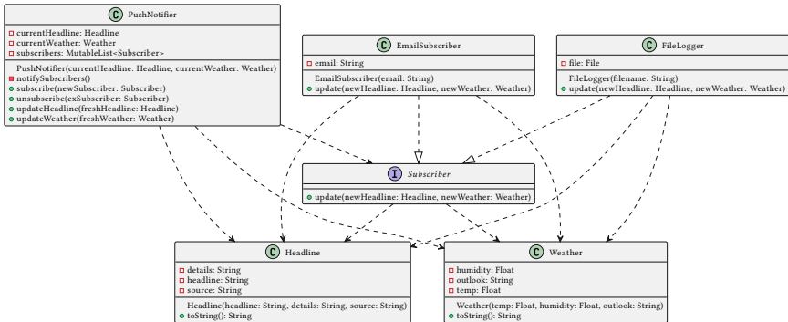
Figure 52: observer example
