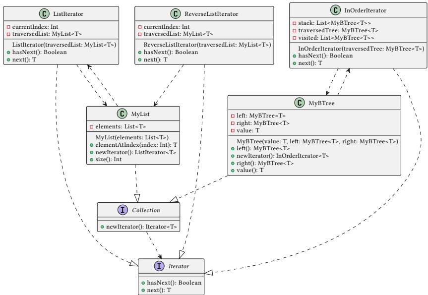
Figure 57: iterator
