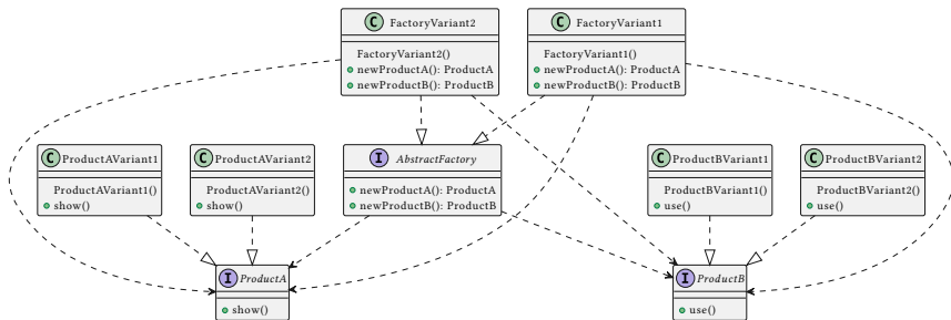
Figure 27: abstract factory
