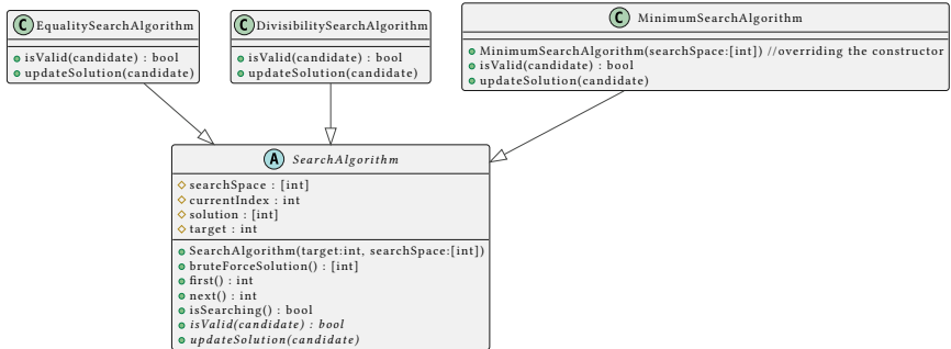
Figure 55: template example
