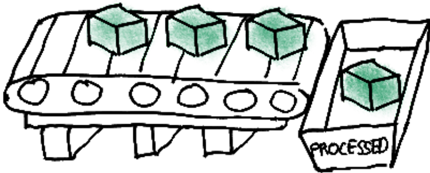
Figure 56: iterator
