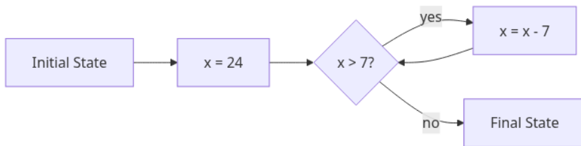
Figure 5: Example Program
