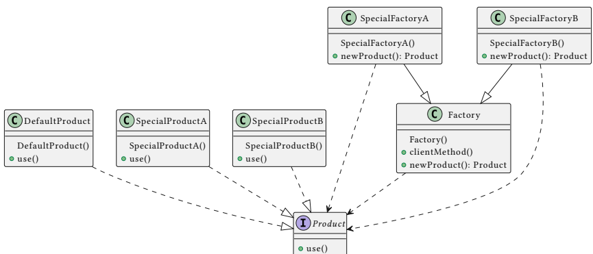
Figure 23: factory method class diagram
