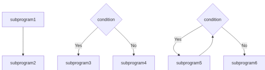
Figure 4: Flowcharts
