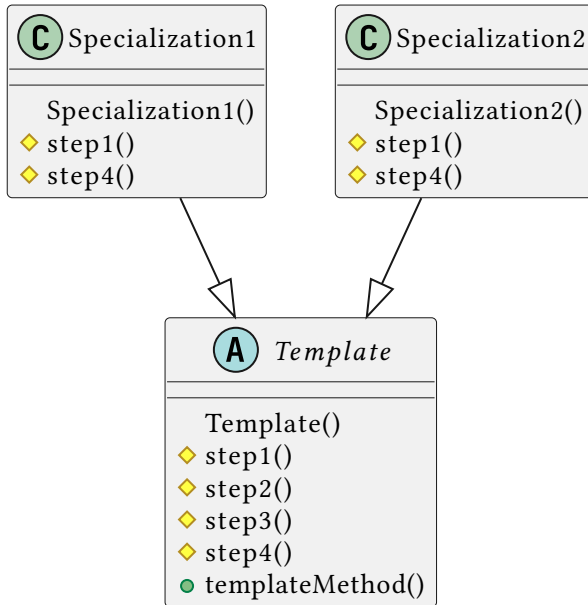
Figure 54: template method
