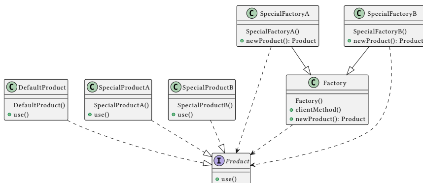
Figure 20: factory method class diagram
