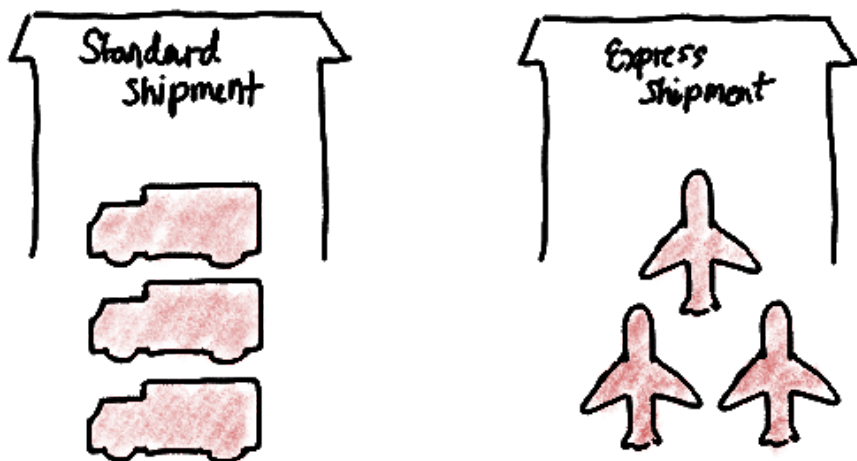
Figure 19: Factory Method
