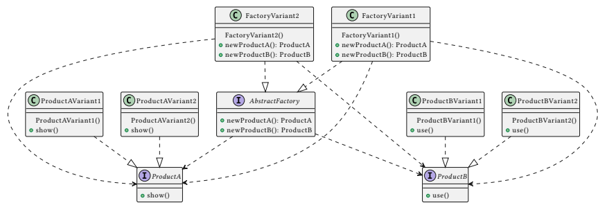
Figure 27: abstract factory
