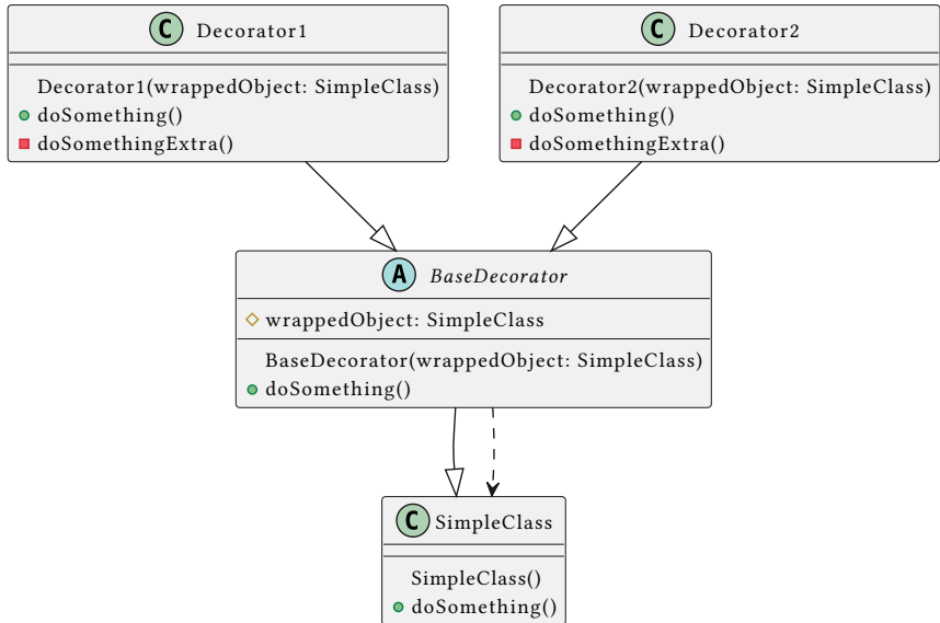
Figure 31: decorator
