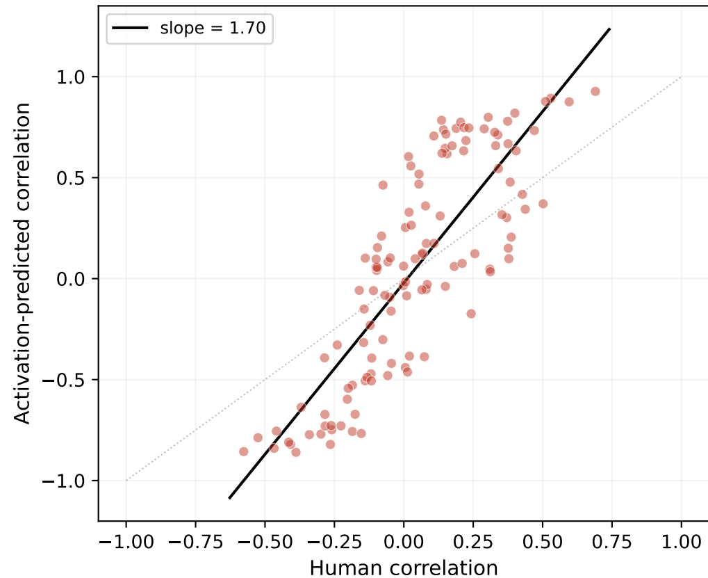
(A) Llama 8B Instruct Mantel r = 0.83 , slope = 1.70
