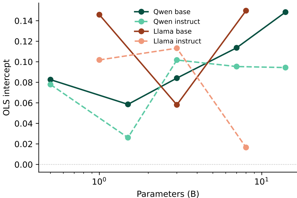
Subscale-level OLS intercept vs model size
