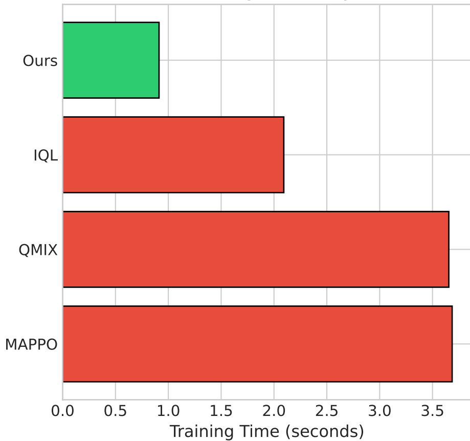
Training Efficiency
