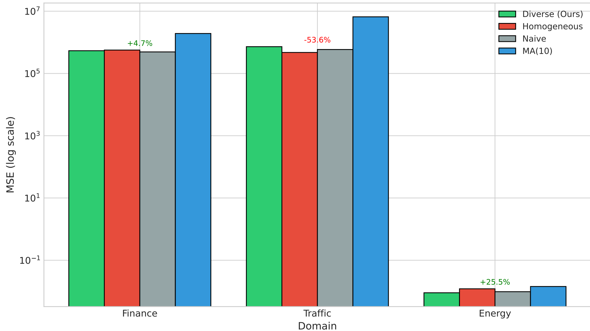
Prediction MSE Across Domains
