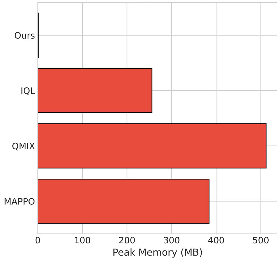
Memory Efficiency
