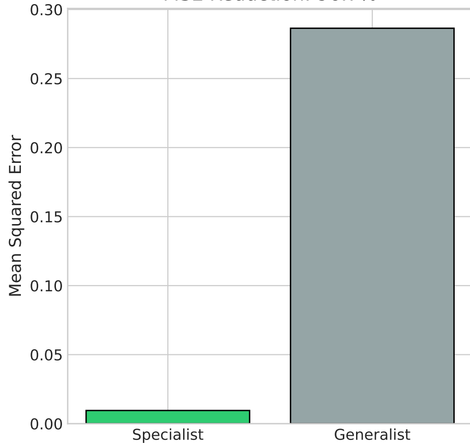
MSE Reduction: 96.7%
