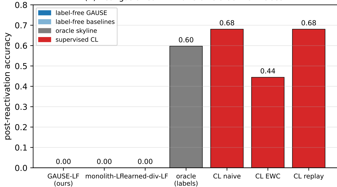
(A) Real gas stream: who retains a dormant class?
