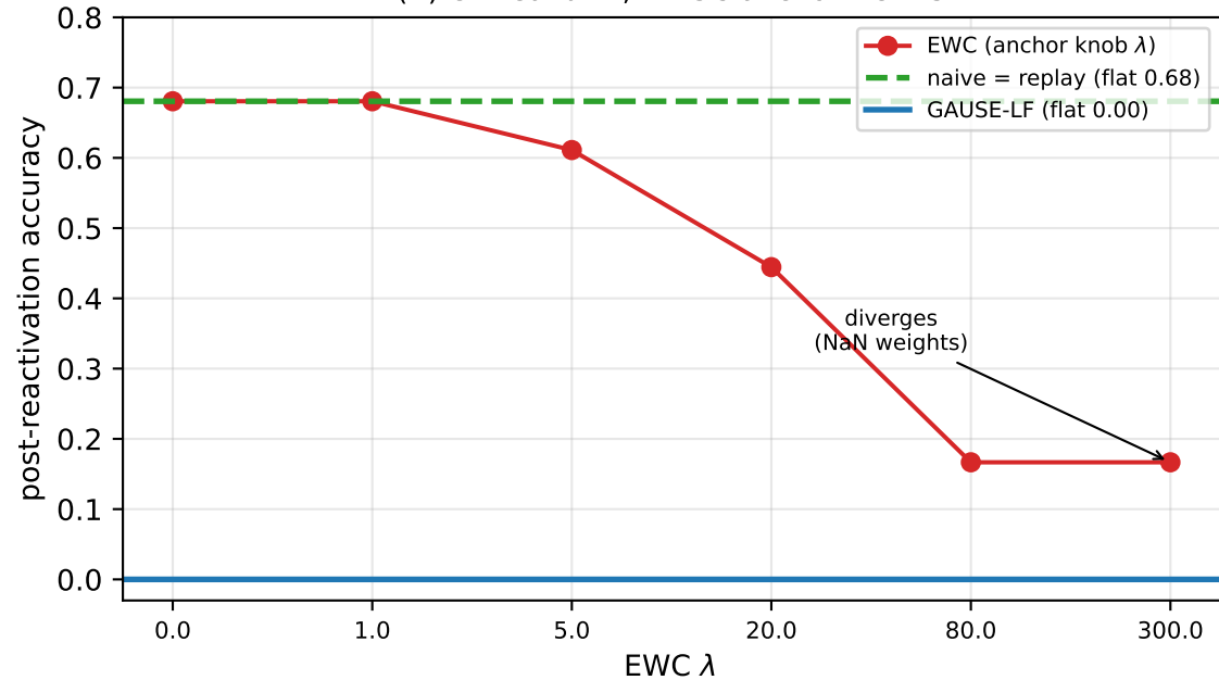
(B) On real drift, EWC's anchor HURTS
