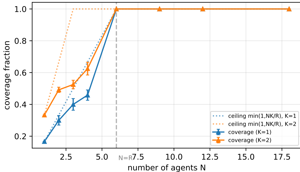
Coverage vs population size
