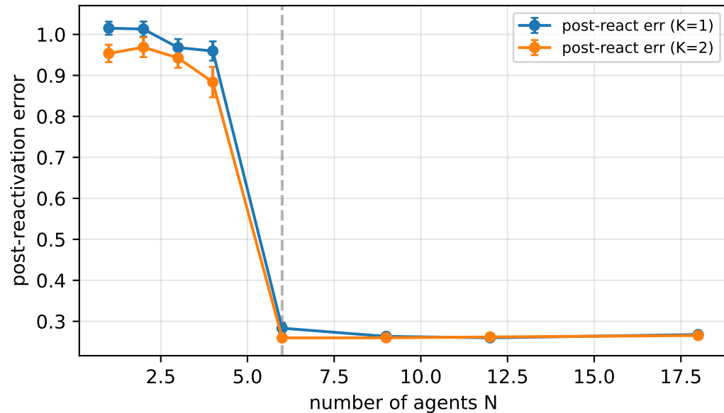
Retention vs population size
