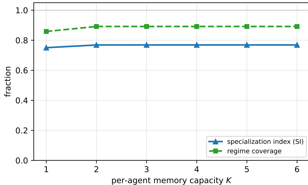
Latent regimes recovered from competence alone
