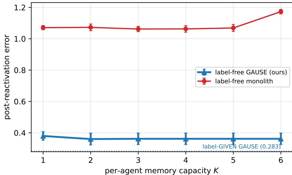
Retention WITHOUT the regime label
