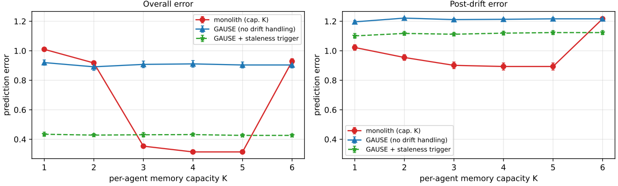
Figure 10 Intra-regime concept drift. Standard GAUSE (blue) pins a stale specialist (overall error 0.90, worse than a relearning monolith); a staleness trigger (green) recovers most of it (0.43). Reward-independent retention helps under dormancy and hurts under drift.
