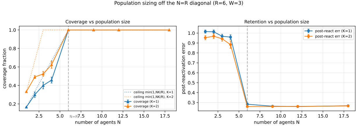
Figure 13 Population sizing off the N \approx R diagonal ( R=6 ). Below N=R , coverage (left) tracks N rather than the feasibility ceiling \min(1, NK/R) and retention (right) degrades; for N \geq R coverage saturates and surplus agents idle ( N - R redundant) without harming retention.
