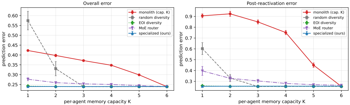
Figure 12 Robustness to the capacity model: the full non-stationary sweep re-run under the soft interference-decay model (no eviction). The reward-independence dissociation survives intact, ruling out an artifact of discrete LRU eviction.
