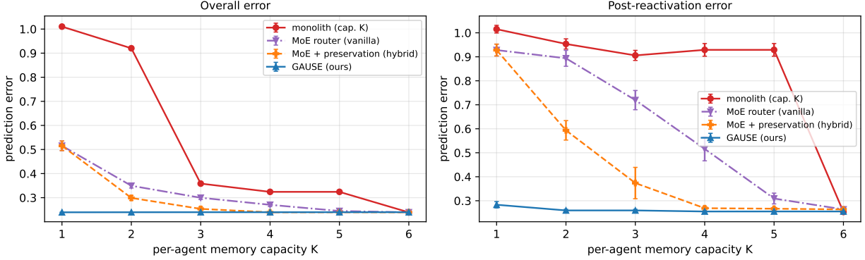
Figure 9 Hybrid arm: reward-driven routing plus a reservation term. It recovers most retention with spare capacity (+48% at K=3 ) but cannot help at K=1 ; the competitive population retains even at K=1 . Reward-independence of protection is the operative property.
