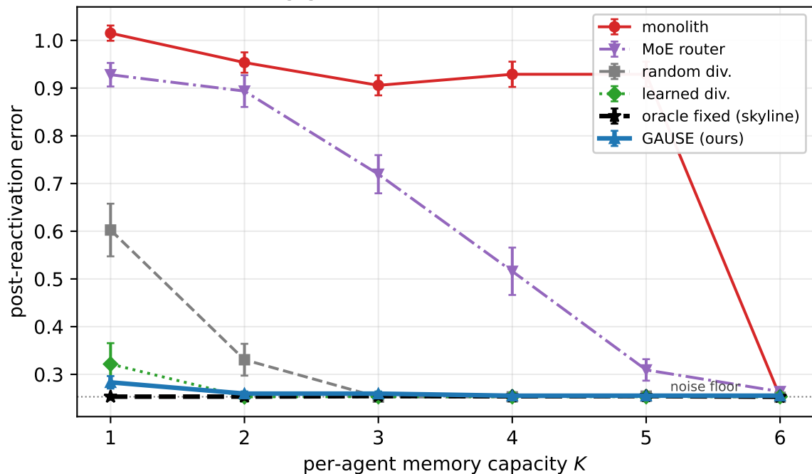
Retention: GAUSE matches the oracle fixed assignment without being given the labels ( R=6 , W=3 , hard LRU)
