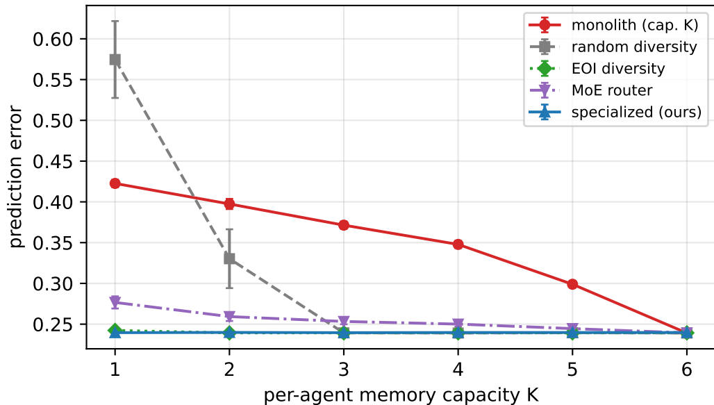
Overall error
