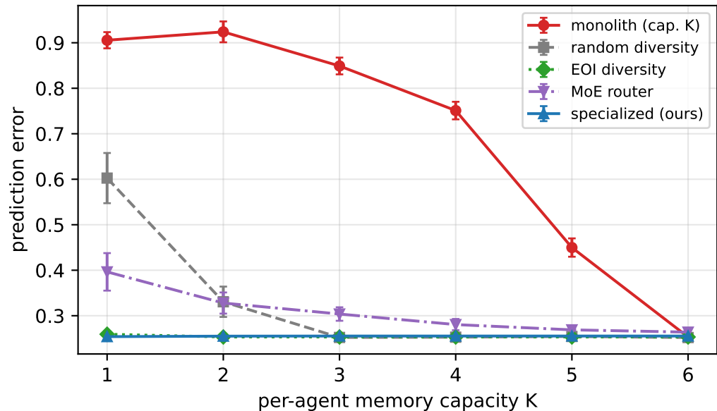
Post-reactivation error
