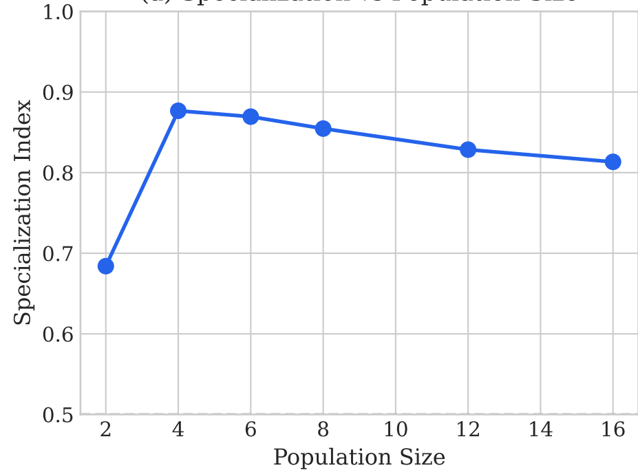
(a) Specialization vs Population Size
