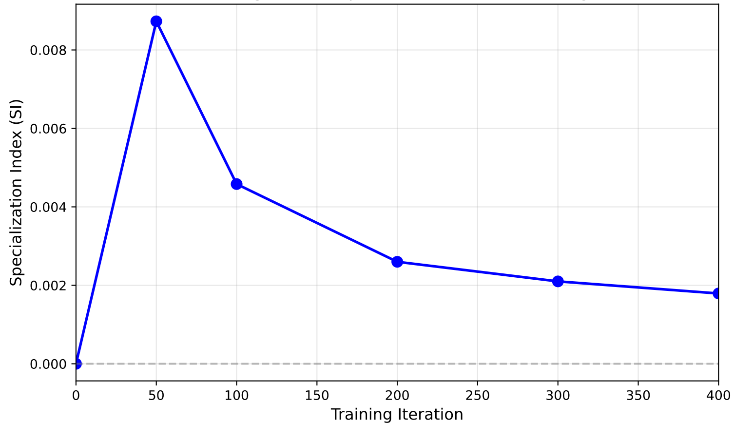
Emergence of Specialization Over Training
