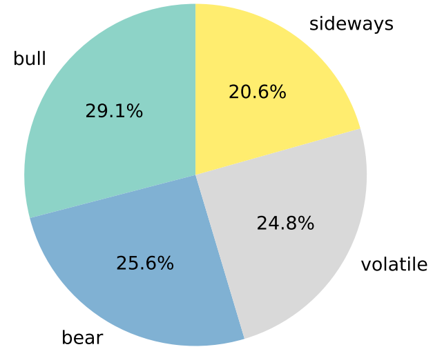
Solar (4 regimes)
