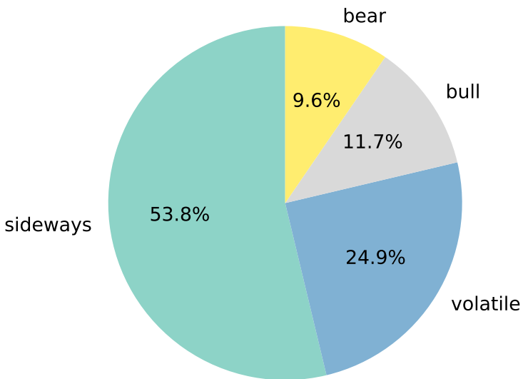
Crypto (4 regimes)
