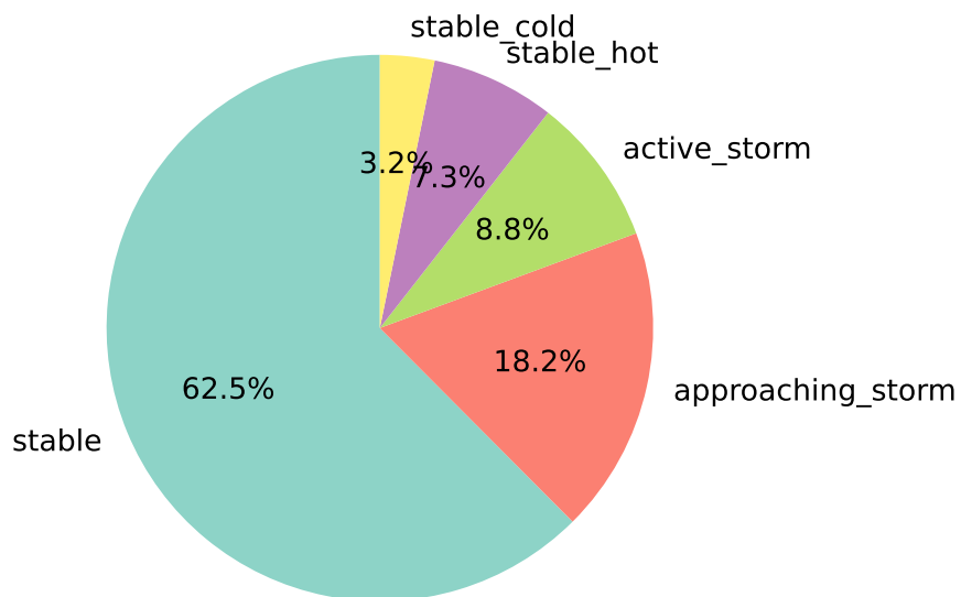
Weather (5 regimes)
