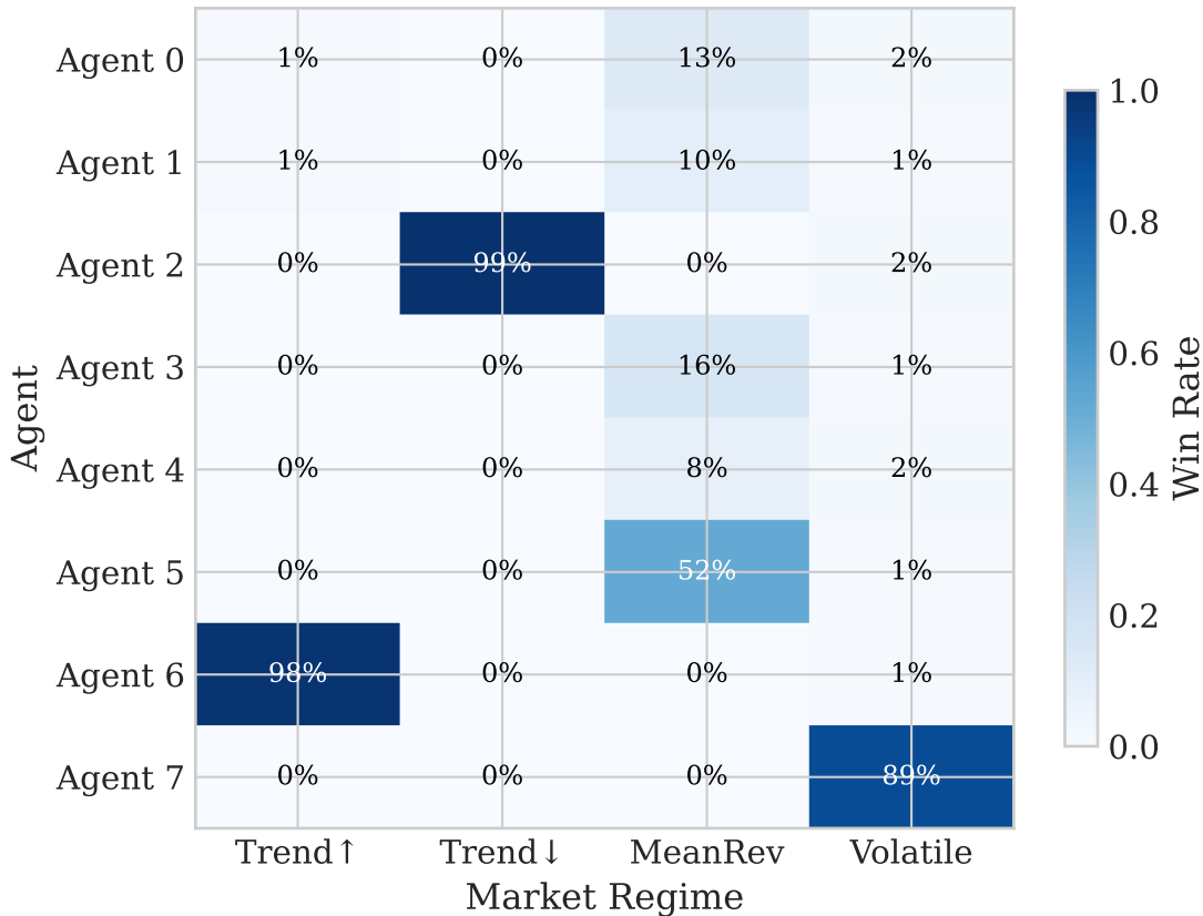
Agent-Regime Win Rate Matrix (Emergent Specialization)
