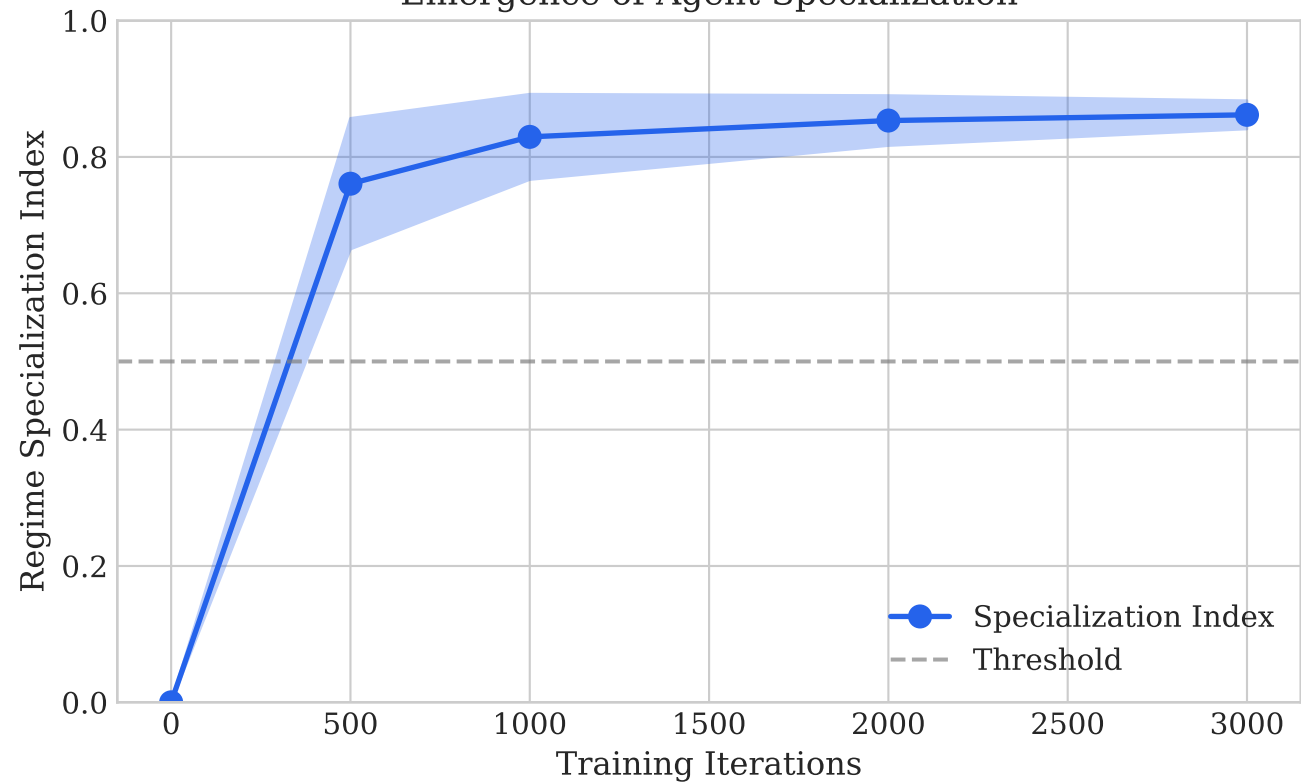
Emergence of Agent Specialization
