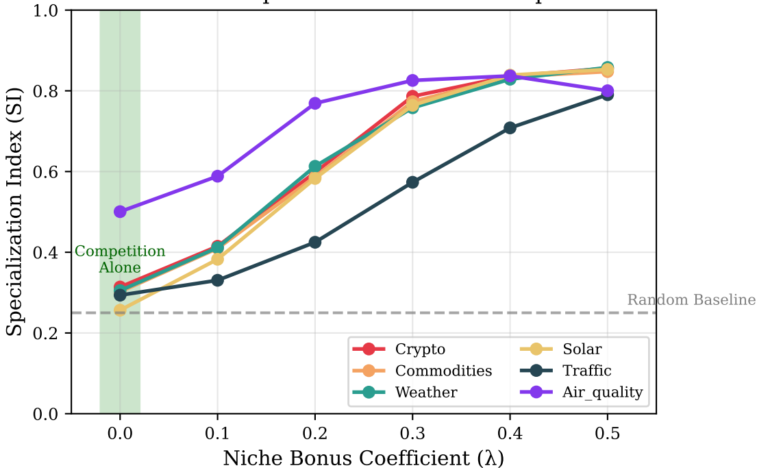
\lambda=0 Ablation: Competition Alone Induces Specialization
