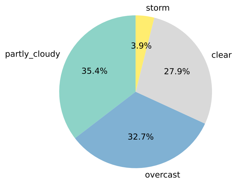
Solar (4 regimes)
