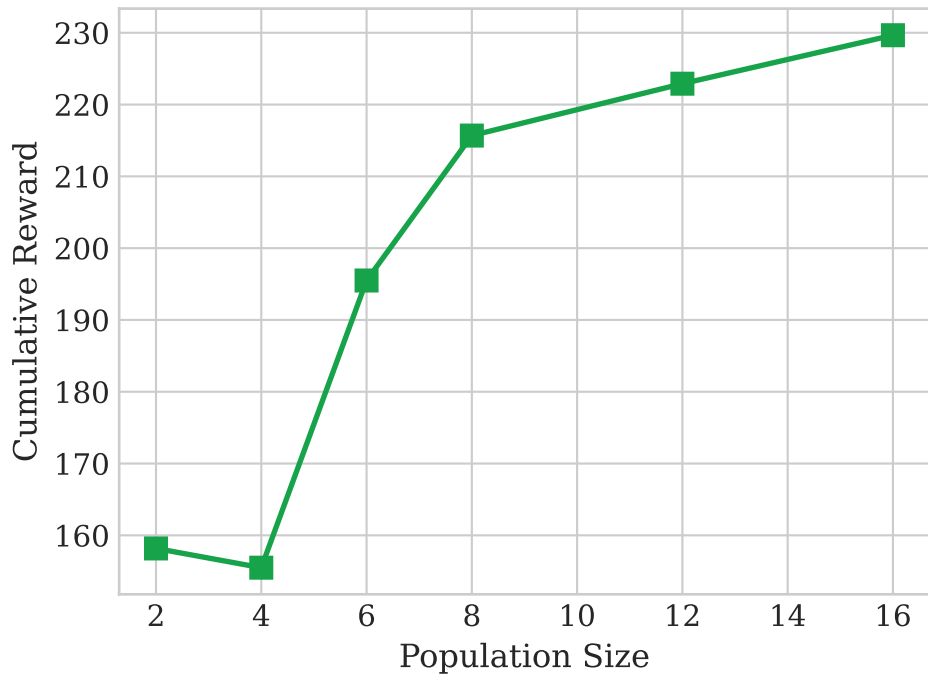
(b) Performance vs Population Size
