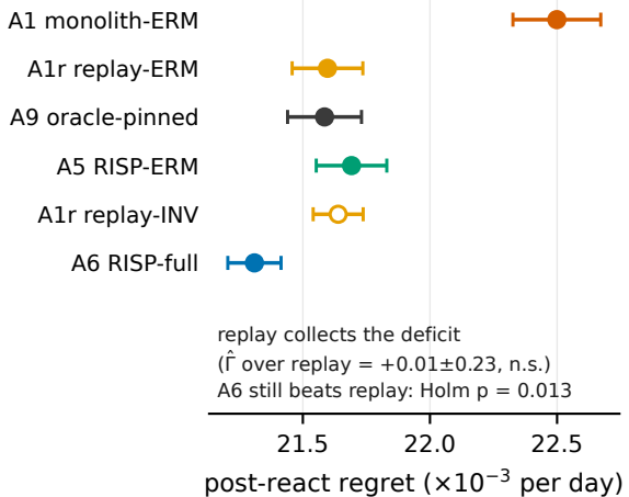
(b) French 49, L3@15% (20 seeds)
