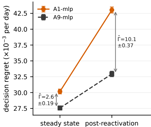
(a) MLP deficit is 3.9\times probe-localized (100 seeds)
