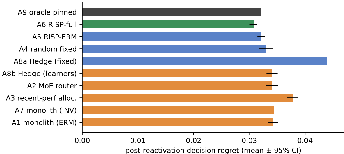
Post-reactivation regret by arm (synthetic, 20 seeds)
