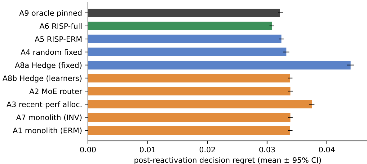
Post-reactivation regret by arm (synthetic, 100 seeds)
