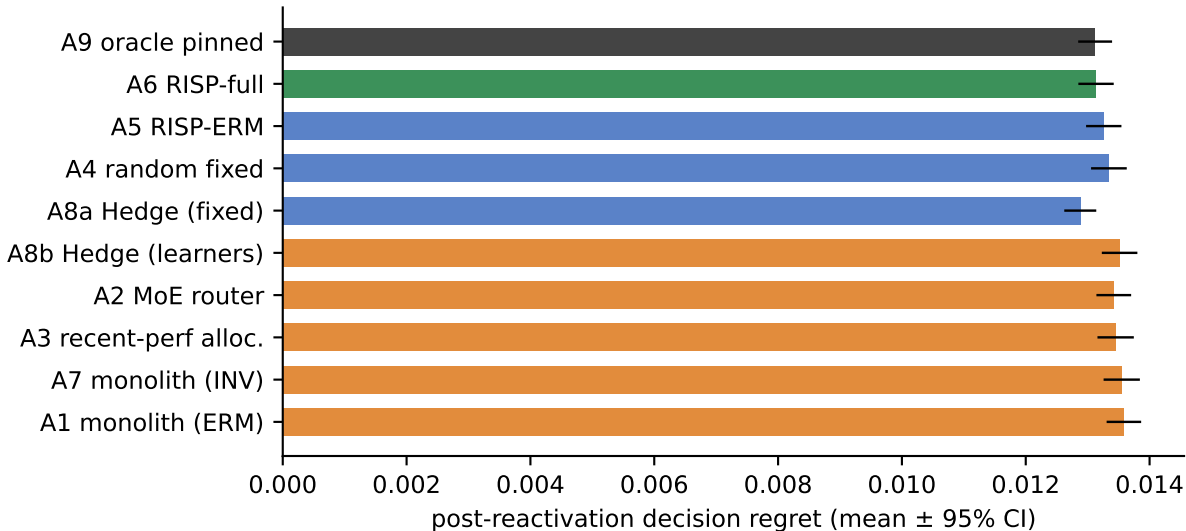
Post-reactivation regret (regime-stitched crypto, 100 seeds)
