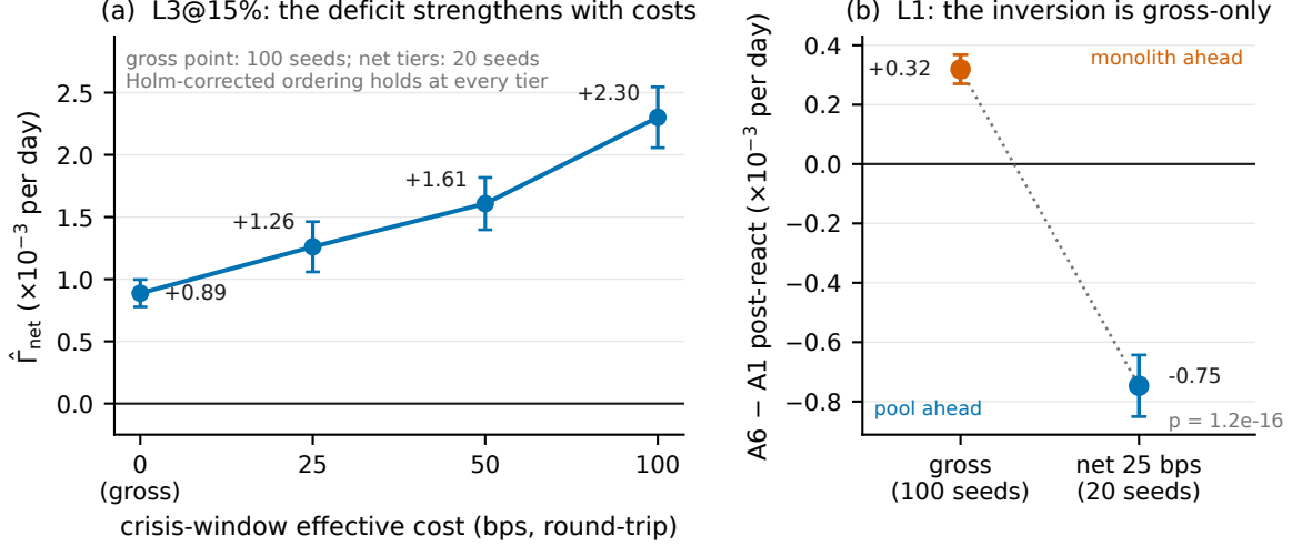
Figure 5: Crisis-window transaction costs, both-pay convention. Left: the L3 deficit \hat{\Gamma} strengthens monotonically with the cost tier (gross point at 100 seeds; net tiers at 20 seeds, annotated). Right: the L1 walk-forward inversion reverses net of 25 bps — the inversion, not the deficit, was the gross-only phenomenon.
