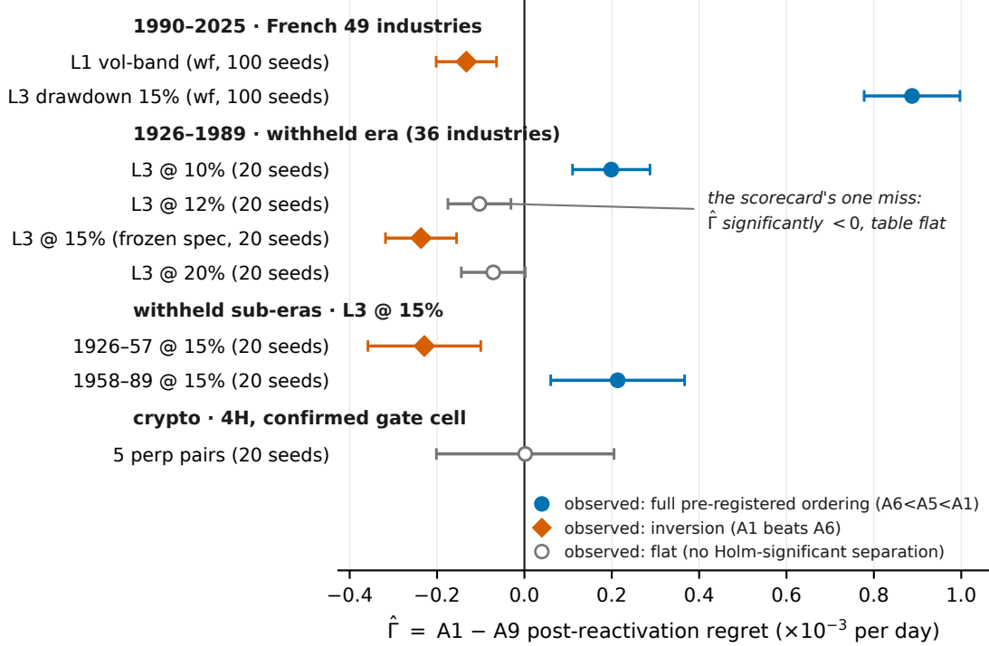
Figure 7: The sign-rule scorecard: \hat{\Gamma} (mean \pm 95% CI) for every scored cell, colored and shaped by the observed outcome (full pre-registered ordering / flat / inversion, classified by the pre-stated rule). Positive deficits coincide with orderings and negative deficits with inversions in both eras; the single miss (12% withheld: negative-significant \hat{\Gamma} , flat table) is annotated. Walk-forward intervals are seed noise conditional on each window’s single history.
