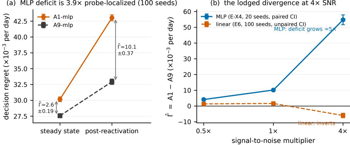
Figure 4: Emergent interference (EIm). Left: under a shared MLP trunk with nothing evicted, the A1–A9 gap is \approx 4\times larger in post-reactivation probe windows than at steady state — a forgetting transient, measured rather than injected. Right: the deficit grows with SNR under gradient descent, diverging from the linear E6 inversion (unpaired CIs for the linear series); the single-readout caveat is discussed in the text.
