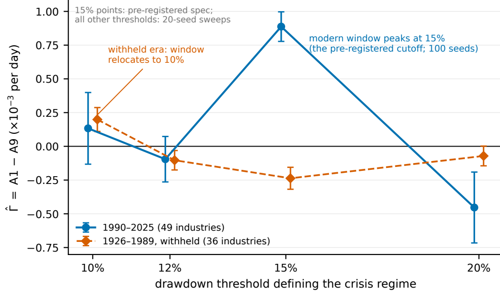
Figure 6: The positive-deficit window relocates across eras: \hat{\Gamma} versus drawdown threshold for 1990–2025 (peak at the pre-registered 15%) and the withheld 1926–1989 era (peak at 10%, where the denser crisis inventory shifts the granularity window). Fragility replicates in pattern, not in location.
