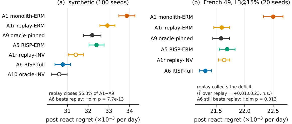
Figure 3: Replay with an eviction-decoupled buffer, both substrates (post-reactivation regret, mean \pm 95% CI). Left: synthetic (100 seeds) — the replay monolith closes 56.3% of the deficit, below the pre-registered 60%, and remains far from A6. Right: French 49 L3 walk-forward (20 seeds) — replay collects the deficit (matching A9) yet the invariance-equipped emergent pool still wins.
