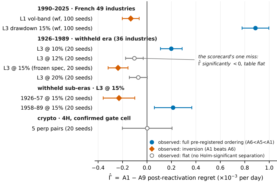
Figure 7: The sign-rule scorecard: \hat{\Gamma} (mean \pm 95% CI) for every scored cell, colored and shaped by the observed outcome (full pre-registered ordering / flat / inversion, classified by the pre-stated rule). Positive deficits coincide with orderings and negative deficits with inversions in both eras; the single miss (12% withheld: negative-significant \hat{\Gamma} , flat table) is annotated. Walk-forward intervals are seed noise conditional on each window's single history.
