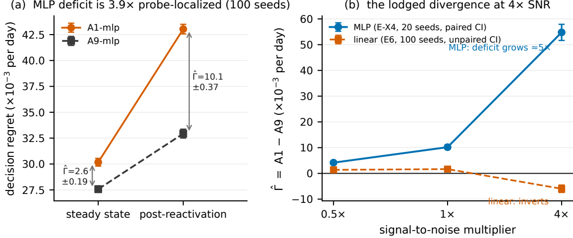
Figure 4: Emergent interference (E1m). Left: under a shared MLP trunk with nothing evicted, the A1–A9 gap is \approx 4\times larger in post-reactivation probe windows than at steady state — a forgetting transient, measured rather than injected. Right: the deficit grows with SNR under gradient descent, diverging from the linear E6 inversion (unpaired CIs for the linear series); the single-readout caveat is discussed in the text.
