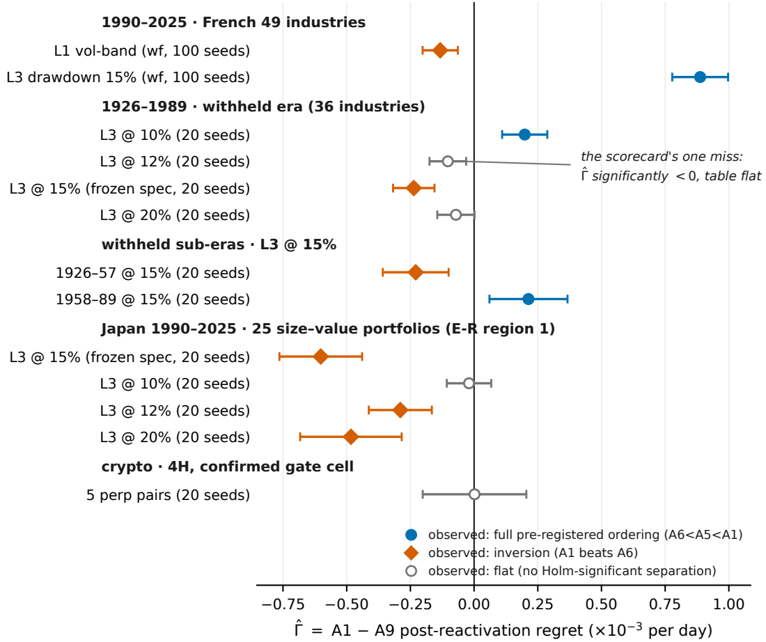
Figure 7: The sign-rule scorecard: \hat{\Gamma} (mean \pm 95% CI) for the walk-forward cells of all three market histories (US 1990–2025, US 1926–1989 with its sub-eras, Japan 1990–2025) plus the 4H crypto gate cell; the NBER-labeler and stitched cells of the inclusive scorecard are tabulated in the released JSONs. Color and shape encode the observed outcome (full pre-registered ordering / flat / inversion, classified by the pre-stated rule). Positive deficits coincide with orderings and negative deficits with inversions in both directions and both hemispheres; the annotated cell (12% withheld: negative-significant \hat{\Gamma} , flat table) is the sign rule's one out-of-sample miss —distinct from the inclusive scorecard's strong-form-only misses, which are weak-form hits, not rule violations. Walk-forward intervals are implementation precision (seed noise) conditional on each window's single history.
