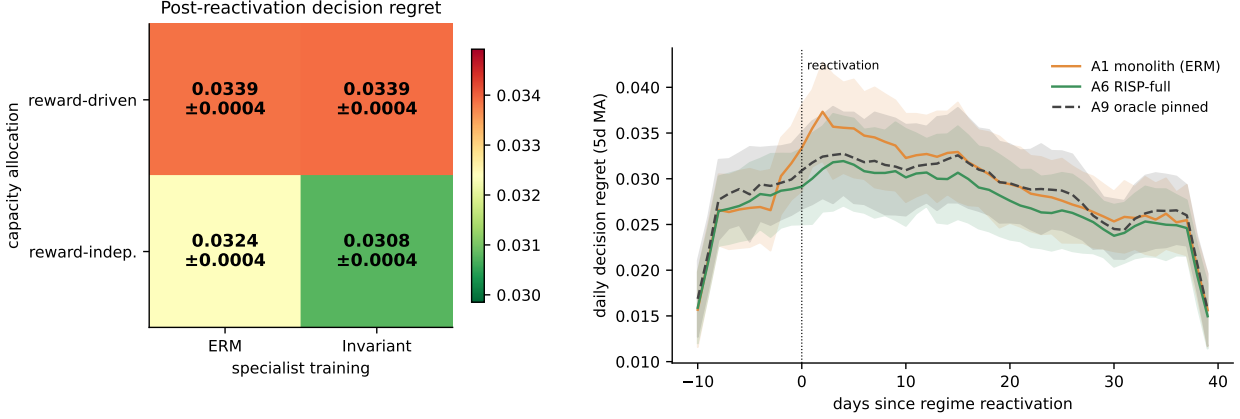
(a) The 2x2: the invariance axis is inert in the reward-driven row (the predicted asymmetry).
