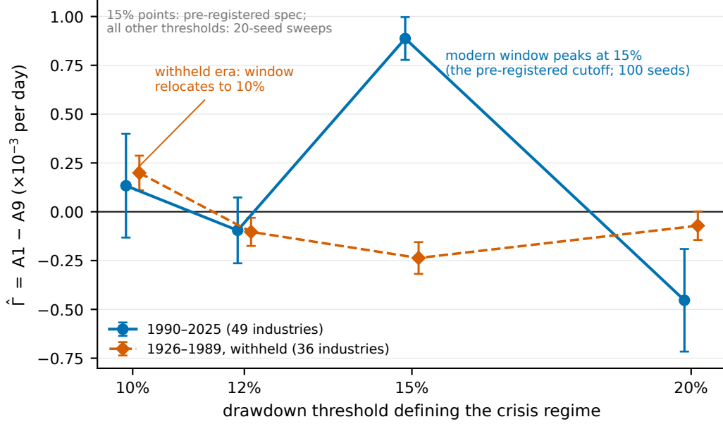
Figure 6: The zero-hysteresis coarse sweep: \hat{\Gamma} versus drawdown threshold for 1990–2025 (peak at the pre-registered 15%) and the withheld 1926–1989 era (peak at 10%). At this register the window appears to relocate with crisis density; the lodged fine map (E-X2, text) adjudicates window on both eras with an overlapping 13–16% band under exit hysteresis, superseding the relocation reading—what this figure shows is the h=0 slice.
