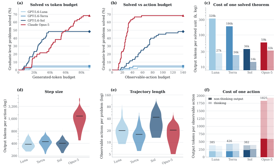
Figure 7: Budget curves and per-problem spend. (a)–(b) Solve rate at the graduate level by token and action budget. (c) Tokens per solved unit. (d) Tokens per action. (e) Actions per problem. (f) Non-thinking and thinking tokens per action. Panels (c) and (f) distinguish the graduate level (saturated) from the research level (lighter); (d)–(e) pool both. GPT thinking counts use reasoning_output_tokens ; Opus uses harness-reported estimates as a lower bound.
