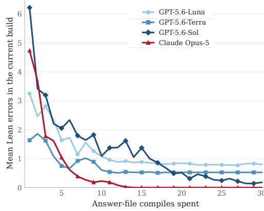
Figure 6: Answer-file error trajectories. Mean Lean errors by compilation count, carrying final counts forward for completed runs. Both graduate and research levels are pooled; runs require at least three answer-file compilations, excluding scratch probes.
