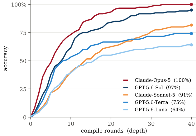
Figure 9: Counterexample accuracy by Lean compilation round. The horizontal axis is truncated at 40 rounds; the values in the legend are the final success rates after all rounds (cf. Table 7).
