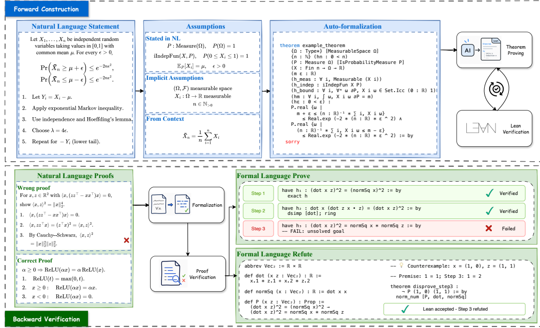
Figure 1: MLP-Bench forward-backward framework: Forward construction (top) covers auto-formalization and theorem-proving. Backward verification (bottom) covers proof verification, localizing the first erroneous step with Lean-checked evidence. Check Section 2 for further details.
