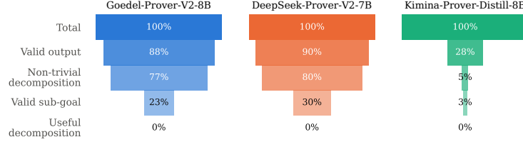
Figure 8: Decomposition funnel on 60 theorems per model; percentages use all 60 attempts.
