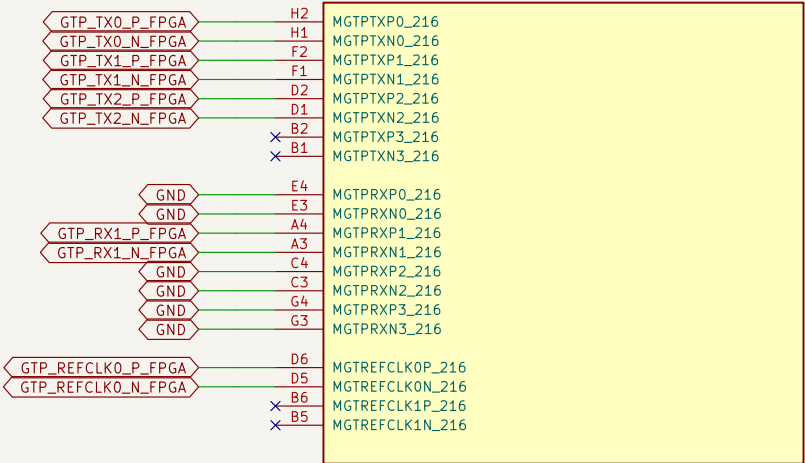
U1C XC7A25T-2CSG325I
