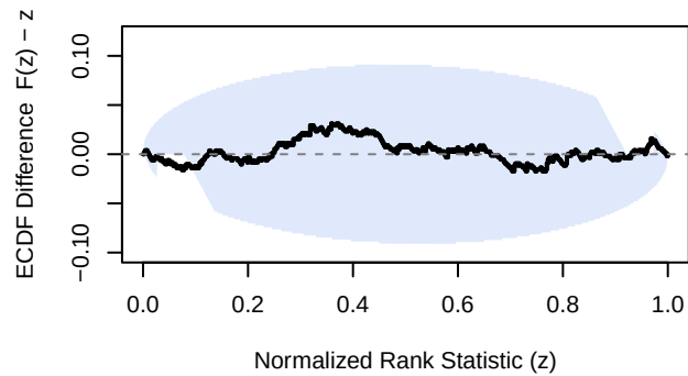
mu - v_IMTRUE
