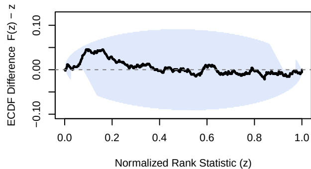
mu - t0
