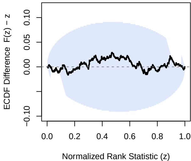
var - t0.t0
