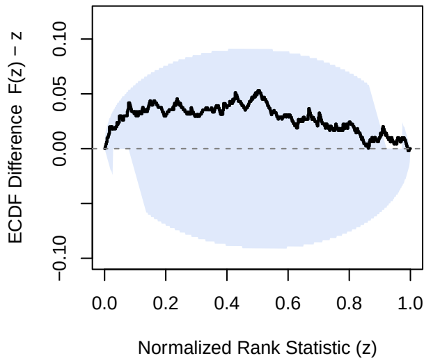
var - m_IMTRUE.m_IMTRUE
