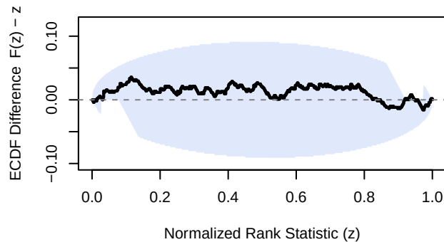
var - t0.t0
