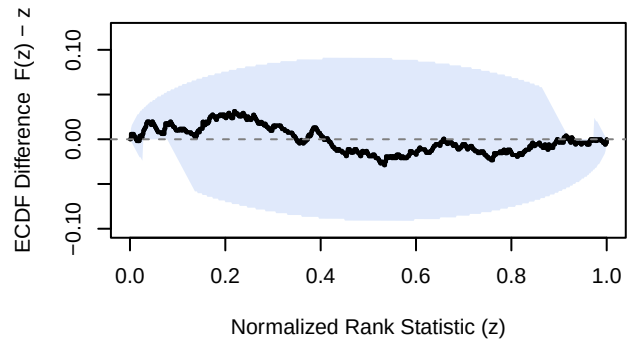
\mu - t0
