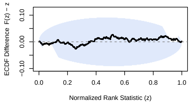
\mu - v\_IMTRUE
