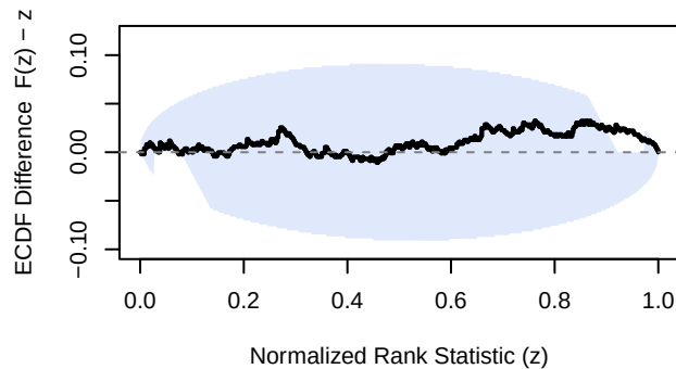
var - v_IMTRUE.v_IMTRUE
