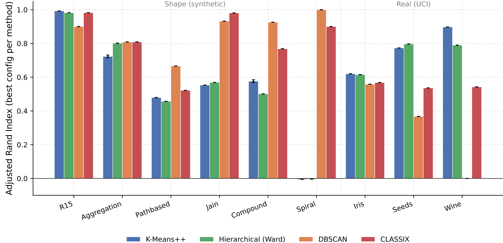
Best clustering quality per dataset across four methods
